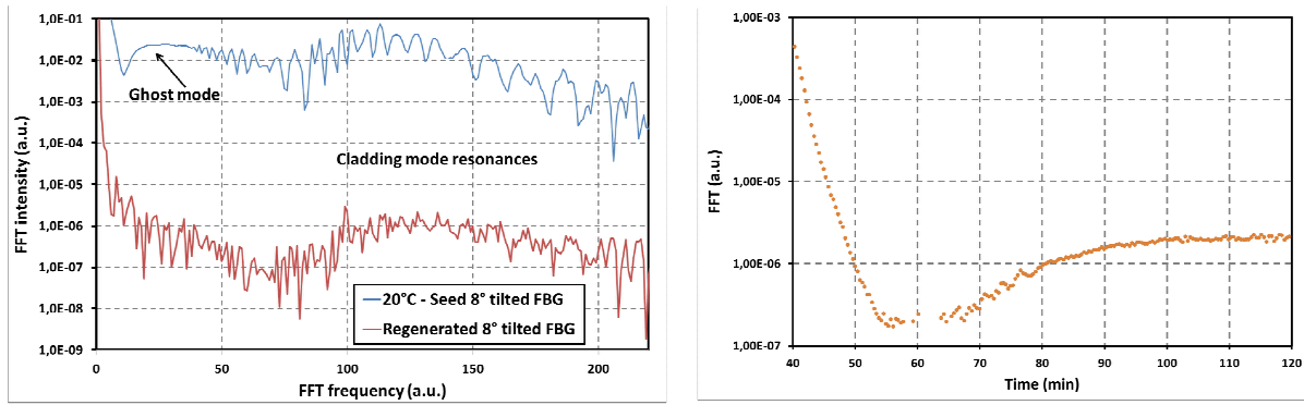
Figure 4. Power spectra for the 8° TFBG before and after regeneration (left). Tracking of the broad peak (located around frequency 140 on the power spectrum graph) attributed to the cladding mode resonances of the 8° TFBG during the regeneration process (right).
