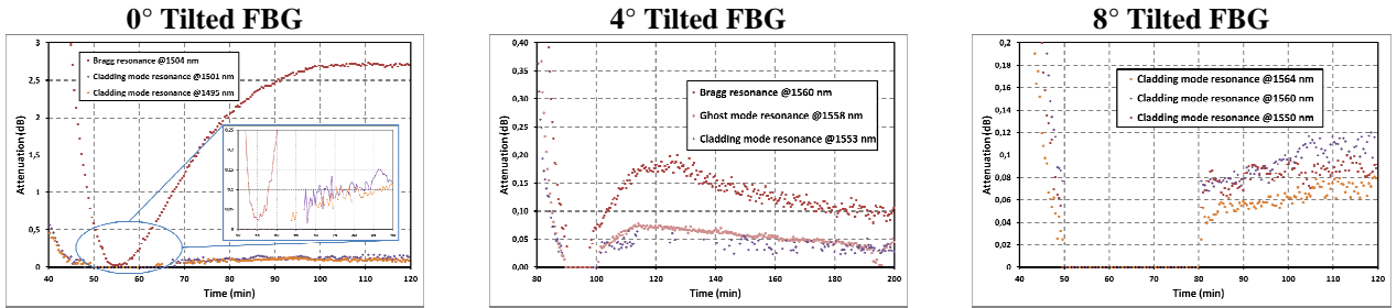
Figure 3. Evolution of distinctive spectral resonances for each Tilted FBG during the regeneration process.
