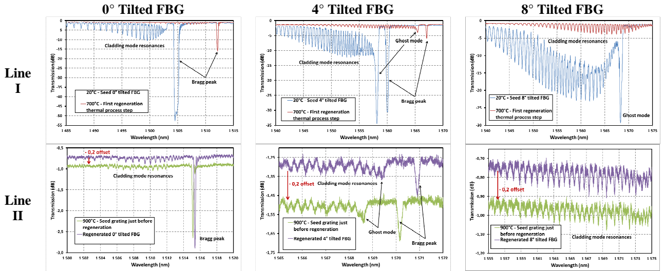
Figure 2. Transmission spectra of the three Tilted FBGs investigated ( 0^\circ , 4^\circ and 8^\circ external tilt angles). Line I: before the regeneration process (in blue) and at the end of the first annealing step at 700^\circ\text{C} (in red). Line II: at the 900^\circ\text{C} annealing step (regeneration phase), few minutes before the complete erasing of the seed grating (in violet) and once regenerated (in green).
