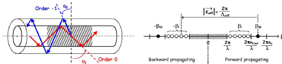
Figure 1. Tilted FBG coupling diagram.
