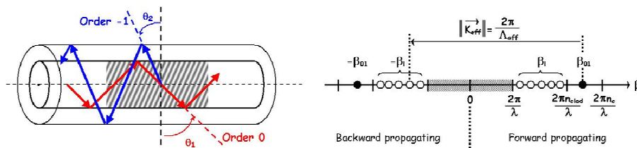
Figure 1. Tilted FBG coupling diagram.
