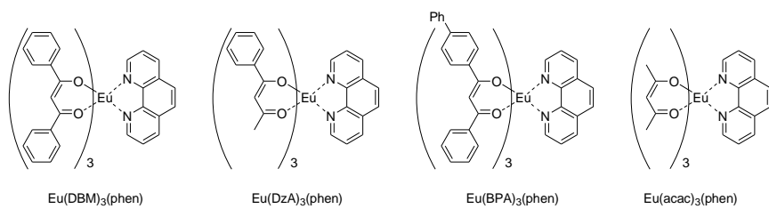
Scheme 11. Europium complexes studied.
