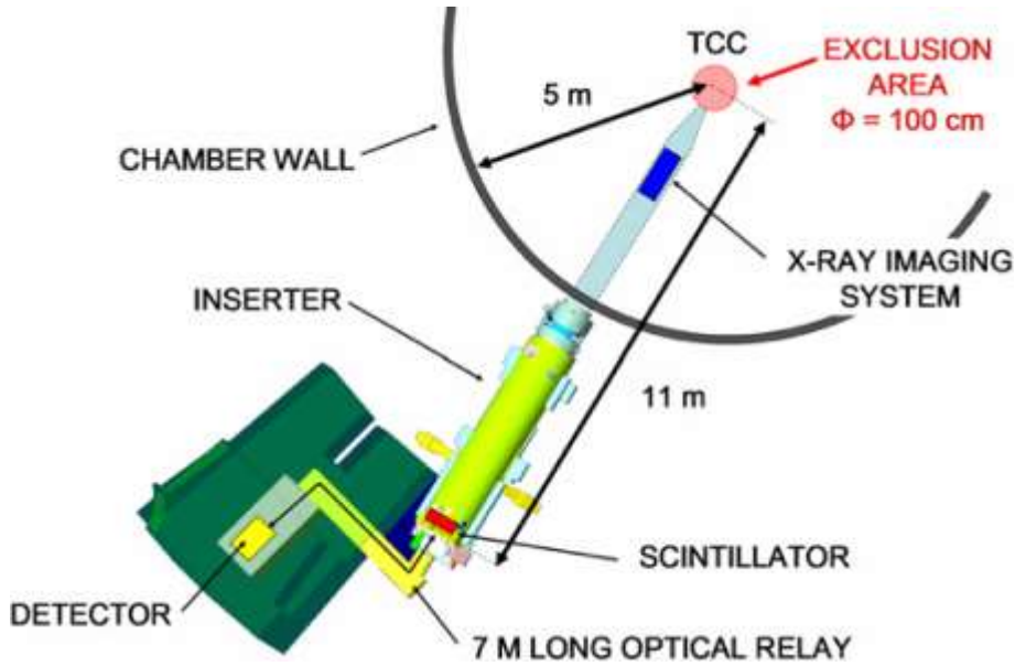
Figure 14. Diagnostic implantation in the LMJ facility.
