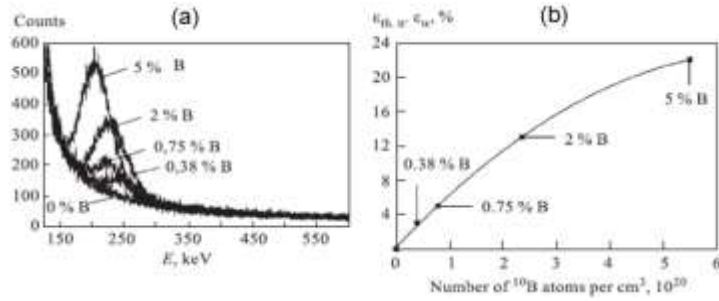
Figure 10. Evolution of neutron sensibility with boron loading (a) on a pulse height spectrum; (b) on a quantic yield versus number of ^{10}\text{B} atom by volume spectra (reproduced with permission from ref 46. Copyright 2001 World Scientific Publishing Company).
