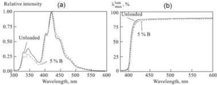
Figure 9. (a) Comparison of photoluminescence spectrum between standard and boron-doped plastic scintillator; (b) Comparison of transmission spectrum between standard and boron doped plastic scintillator (reproduced with permission from ref 44. Copyright 2001 World Scientific Publishing Company).
