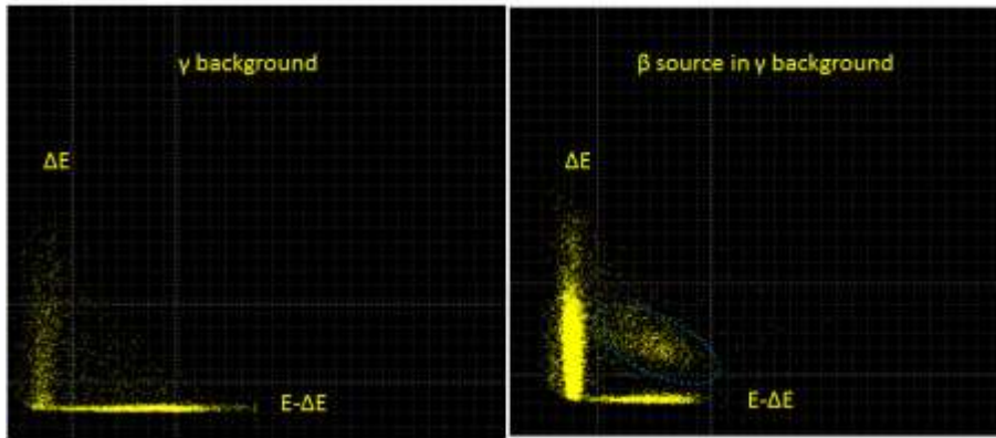
Figure 19. Results of \beta/\gamma discrimination in a phoswich scintillator with a 700 \mu\text{m} thin layer.
