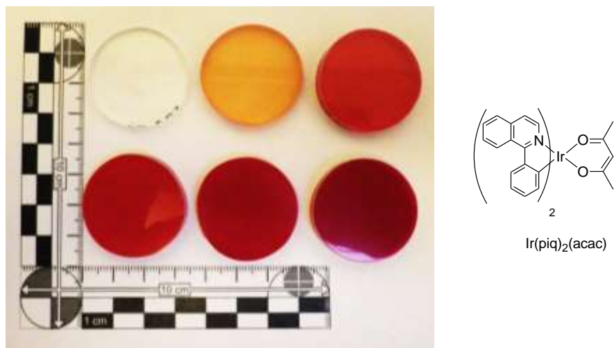
Figure 29. Cross-linked scintillators with increasing loading of Ir(piq) 2 (acac) (0 – 0.1 wt%).
