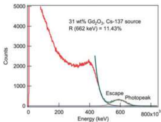
Figure 12. Pulse height spectra of ^{137}\text{Cs} with a plastic scintillator loaded with Gd_2O_3 nanoparticles. (Reproduced with permission from ref 51. Copyright 2013 Royal Society of Chemistry).
