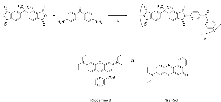
Scheme 5. Synthesis of polyimide (up) and red dyes used as dopant (bottom).
