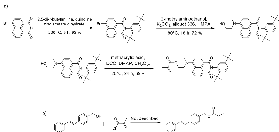
Scheme 10. Synthesis of emitters linked to methacrylic monomer: (a) 1,8-Naphthalimide dye, 68 (b) Stilbene dye. 69
