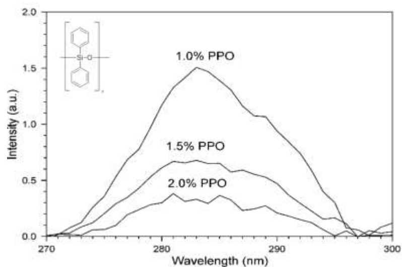
Figure 3. Emission spectra in the UV range ( \lambda_{\text{ex}} = 250 nm) from the diphenylsiloxane unit of a standard siloxane matrix with different PPO concentrations (reproduced with permission from ref 17a. Copyright 2010 from the Authors).
