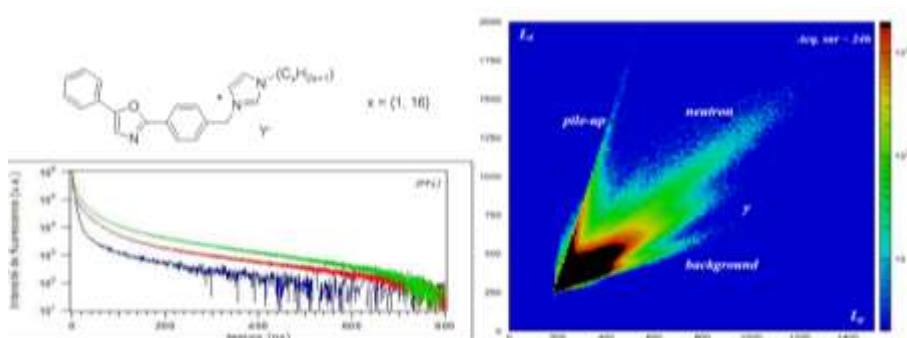
Figure 30. Top left: general structure of ionic liquids allowing PSD between fast neutrons and gamma; bottom left: scintillation decay profiles of OxImC 16 -PF 6 (x = 16; Y = PF 6 ) under gamma excitation (blue), 2 MeV protons (red) and 2 MeV alphas (green). Right: example of PSD biparametric spectrum obtained from the same compound (reproduced with permission from ref 98b. Copyright 2011 from the Author).
