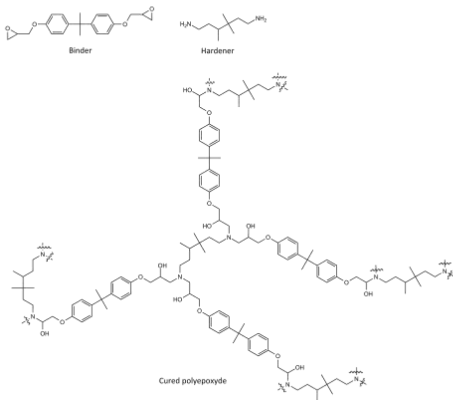
Scheme 3. An example of standard binder and hardener and their subsequent cured polyepoxy.
