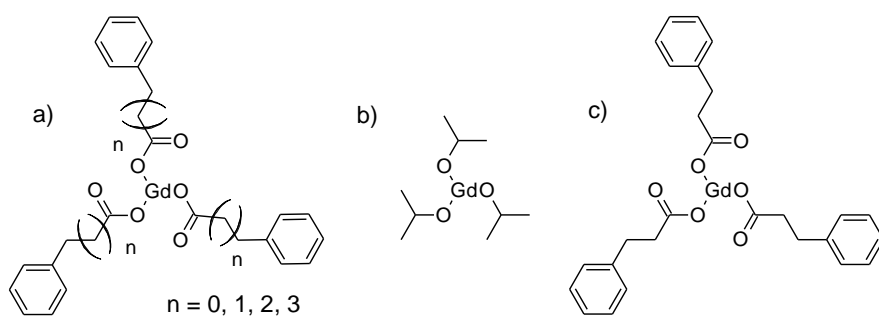
Scheme 6. Organo-gadolinium compounds soluble in classical monomers (MMA and Styrene) a) General formula of gadolinium phenyl-carboxylate; 48 b) Gadolinium isopropoxide; 46 c) Gadolinium phenyl-propionate. 50
