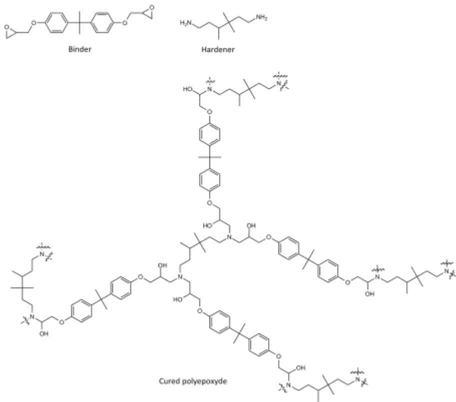
Scheme 3. An example of standard binder and hardener and their subsequent cured polyepoxyde.
