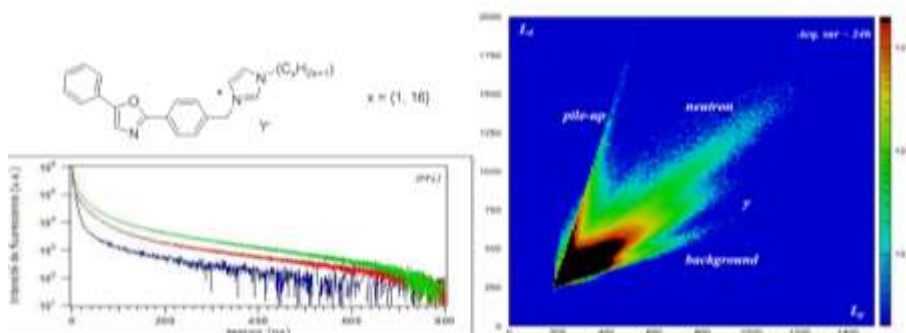
Figure 30. Top left: general structure of ionic liquids allowing PSD between fast neutrons and gamma; bottom left: scintillation decay profiles of OxImC 16 - PF 6 ( x = 16 ; Y = \text{PF}_6 ) under gamma excitation (blue), 2 MeV protons (red) and 2 MeV alphas (green). Right: example of PSD biparametric spectrum obtained from the same compound (reproduced with permission from ref 98b. Copyright 2011 from the Author).
