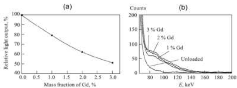
Figure 11. Evolution of neutron sensibility with Gadolinium loading (a) on a light output versus mass fraction spectra; (b) on a pulse height spectra (reproduced with permission from ref 46. Copyright 2001 World Scientific Publishing Company).
