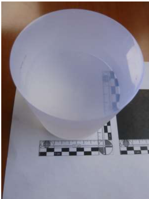
Figure 34. Picture of highly concentrated fluorophore, large plastic scintillator for n/ \gamma discrimination (dimensions \text{\O} 103 \text{ mm} \times \text{h } 114 \text{ mm} , copyright 2013 CEA).
