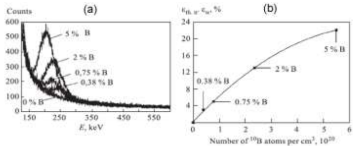
Figure 10. Evolution of neutron sensibility with boron loading (a) on a pulse height spectrum; (b) on a quantic yield versus number of ^{10}B atom by volume spectra (reproduced with permission from ref 46. Copyright 2001 World Scientific Publishing Company).
