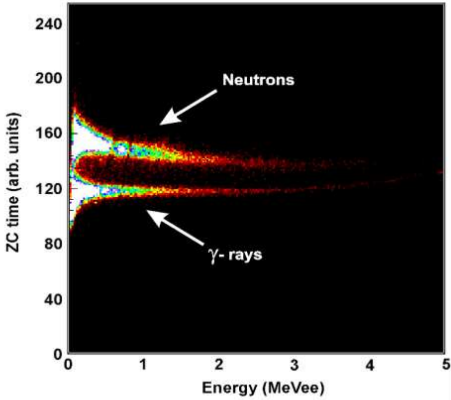
Figure 24. 2D plot of zero crossing time vs. energy measured with composite p -terphenyl based scintillator (50 × 25 mm) under irradiation of a shielded PuBe source (reproduced with permission from ref 84c. Copyright 2012 IOP Publishing).
