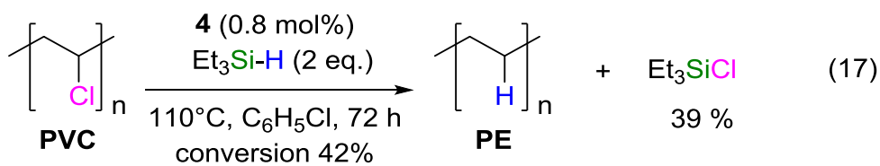
Scheme 6: Reductive dechlorination of PVC to PE with the system 4 / \text{Et}_3\text{SiH} .
