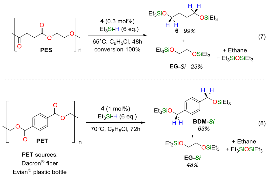
Scheme 3: Reductive depolymerization of PES , and PET with \text{Et}_3\text{SiH} and catalyst 4
