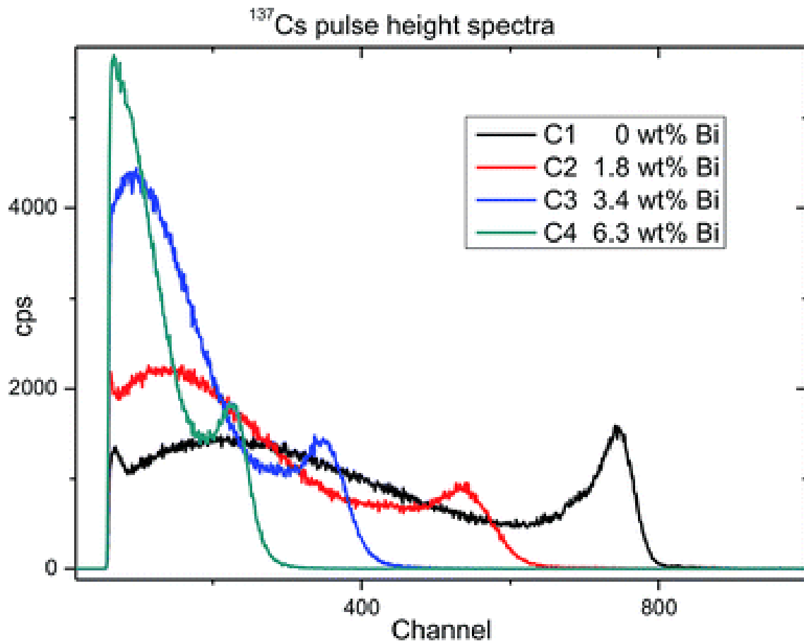
Figure 4 : Pulse height spectra of Bi loaded plastic scintillators
