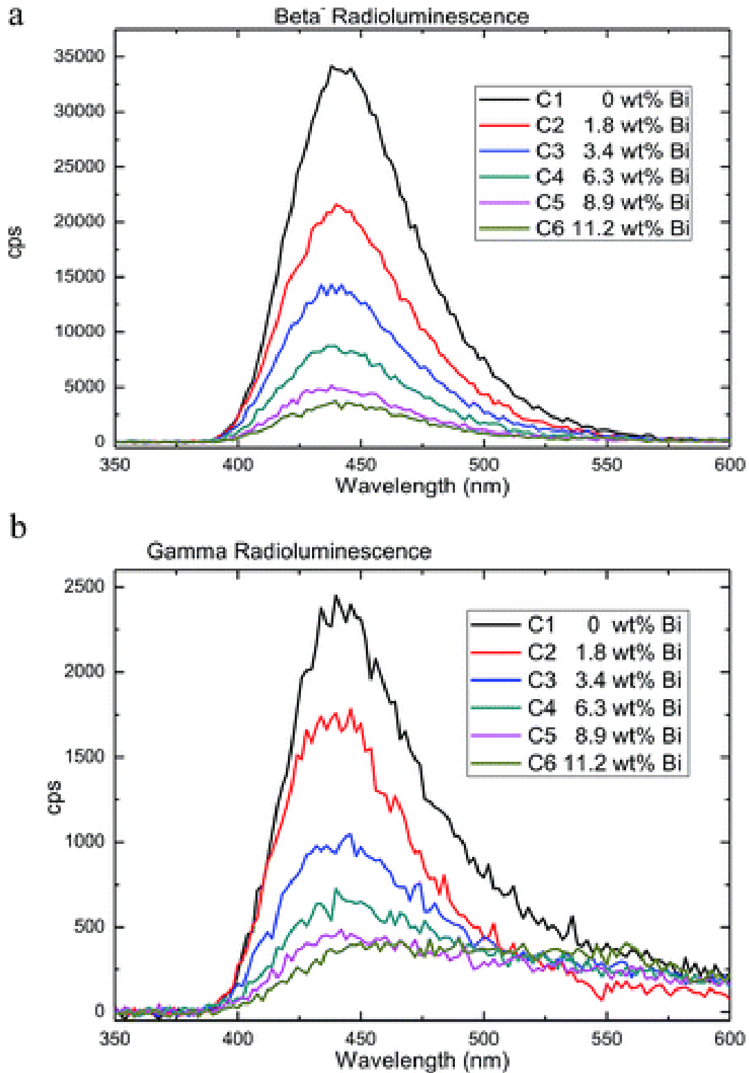
Figure 3 : Radioluminescence experiment on bismuth loaded plastic scintillators with (top) ^{90}\text{Sr}/^{90}\text{Y} (25 MBq) beta source and (bottom) ^{137}\text{Cs} (206 kBq) gamma source
