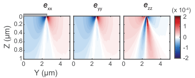
FIG. 6. Finite-element COMSOL simulations of the strain tensor components along the principle crystal axes x \parallel [100] , y \parallel [010] and z \parallel [001] and their variation as a function of position in the device. A cross-section of the aluminium wire (drawn to scale) is represented by the grey gradient-filled box above the silicon substrate (which bounds the strain data). Only half of the wire is displayed here due to it being symmetric about its center. Here the xyz crystal axes are related to the sample frame XYZ (used to describe \delta B_1 and the orientation of B_0 ) by a 45^\circ rotation about Z (see Fig. 1a). We show the result for the wire running parallel to the [110] (or X ) axis, the direction in which the sample was cleaved.
