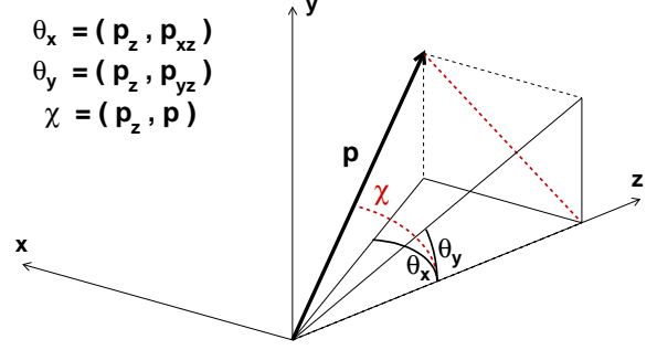
FIG. 2. Variables (p, \theta_x, \theta_y) in the case of a momentum such that p_z > 0 . \theta_x and \theta_y are the diffraction angles and \chi is the deflection angle. \mathbf{p}_z , \mathbf{p}_{xz} and \mathbf{p}_{yz} are respectively the projections of the vector \mathbf{p} on the z axis and on the planes (x, z) and (y, z) .
