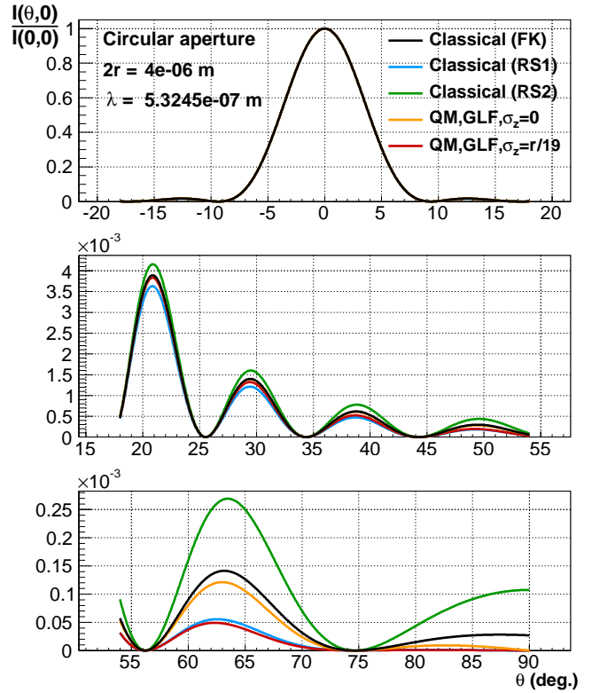
FIG. 5. Comparison of the relative intensities in Fraunhofer diffraction as a function of the diffraction angle in the horizontal plane for a circular aperture of diameter 2r = 4 \mu\text{m} and a monochromatic incident wave corresponding to photons of wavelength \lambda = 532.45 \text{ nm} (KTP Laser). The curves are different from those of Fig. 4 because the experimental parameters are different (shape and size of the aperture, wavelength). However, the gaps between them are the same (except for \sigma_z = r/19 ) because they depend only on the diffraction angle. The value \sigma_z = r/19 was chosen so that the quantum curve is close to the RS1 curve. Moreover, for this value, the damping is less important than that of Fig. 4 because the value r/19 is closer to zero than the value a/10 .
