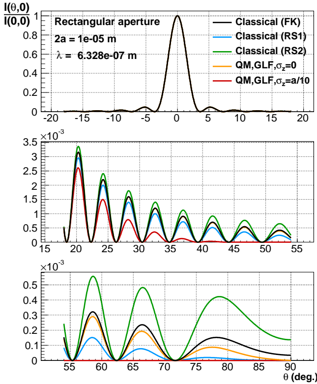
FIG. 4. Comparison of the relative intensities in Fraunhofer diffraction as a function of the diffraction angle in the horizontal plane for a rectangular slit of width 2a = 10 \mu\text{m} and a monochromatic incident wave corresponding to photons of wavelength \lambda = 632.8 \text{ nm} (Helium-Neon Laser). Five theoretical predictions corresponding to the theories of Fresnel-Kirchhoff (FK) and Rayleigh-Sommerfeld (RS1 and RS2) and two quantum predictions corresponding to two values of the standard deviation \sigma_z associated with a Gaussian longitudinal filtering (GLF, \sigma_z = 0 and \sigma_z = a/10 ). The value \sigma_z = 0 corresponds to the case where the diffracted wave associated with the particle is emitted from the wavefront at the aperture whereas a non-zero value corresponds to the case where several wavefronts contribute with different weights and this generates a damping increasing with \theta and \sigma_z .
