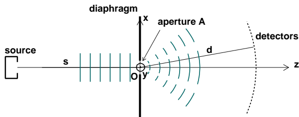
FIG. 1. Schematic representation of experimental setup (section in the horizontal plane (Ox, Oz) ).
