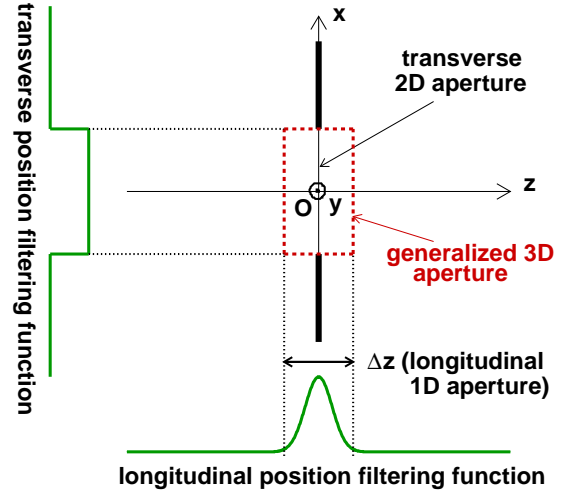
FIG. 3. Example of generalized 3D aperture (section in the (Ox, Oz) plane) and corresponding transverse and longitudinal position filtering functions, whose product is the (joint) position filtering function.
