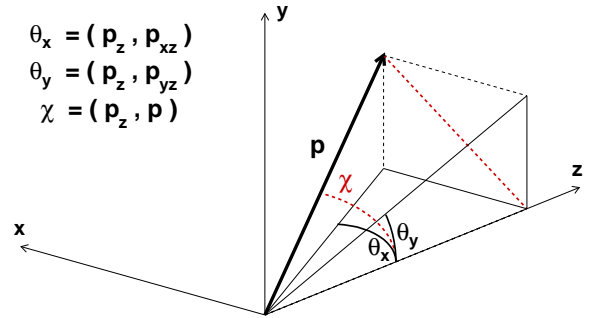
FIG. 2. Variables (p, \theta_x, \theta_y) in the case of a momentum such that p_z > 0 . \theta_x and \theta_y are the diffraction angles and \chi is the deflection angle. \mathbf{p}_z , \mathbf{p}_{xz} and \mathbf{p}_{yz} are respectively the projections of the vector \mathbf{p} on the z axis and on the planes (x, z) and (y, z) .
