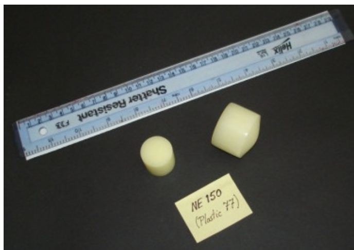
Figure 10: Picture of a degraded NE-150 plastic scintillator (© F.D. Brooks, with permission).
