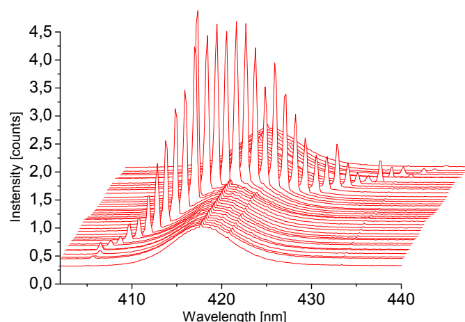
Fig. 8. Variation of the DFB peak wavelength with corotation linear stage position for Ultima Gold™ AB. The interfering angle is directly linked to the the position of the linear translation stage (coupled to both mirror axes). The decrease in peak intensity circa 428 nm is due to non-optimized structuration. DFB excitation beam: tripled (355 nm) pulsed picosecond Nd 3+ :YAG laser.
