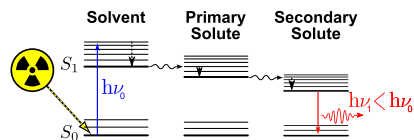
Fig. 16. Typical energy transfer in absorption/emission spectra in a ternary scintillator cocktail.
