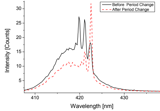
Fig. 13. Coexistence of semi-permanent and dynamic gratings after changing dynamic grating's period. The period changed occurred after a long excitation time and high input power. The semi-permanent grating disappeared shortly after the measurement was taken.
