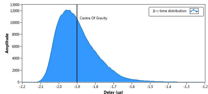
Fig. 11. The time-delay distribution between beta and gamma pulses for a ^{60}\text{Co} source measured in a 4\pi\beta\text{-}\gamma configuration at ENEA. The beta channel used was an atmospheric proportional counter and the gamma channel comprised an NaI(Tl) detector. The digitizer used was a CAEN DT5720.
