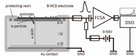
Fig. 5. A schematic view of the SG-BNCD/SiPIN sensor and associated signal processing electronics
