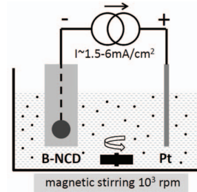
Fig. 4. The experimental arrangement used for electro precipitation of actinides ions onto the CG-BNCD/Si and SG-BNCD/SiPIN sensors
