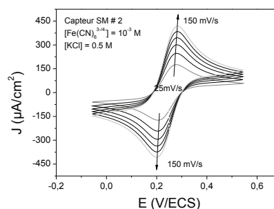
Fig. 3. Cyclic voltammetry curves performed with the CG-BNCD/Si sensor showing the electrochemical activity of the BNCD layer. The measurements are performed using an equimolar solution of potassium ferro-ferricyanide 10^{-3} \text{ M} (outer sphere redox couple) with KCl as supporting electrolyte.
