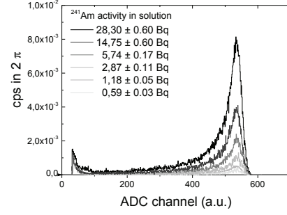
Fig. 7. Pulse-height spectra for varying concentrations of 241 Am in a 100 ml water solution measured with a CG-BNCD/Si sensor. Total activities of the solution were calibrated with a liquid scintillation technique and are indicated in the graph.
