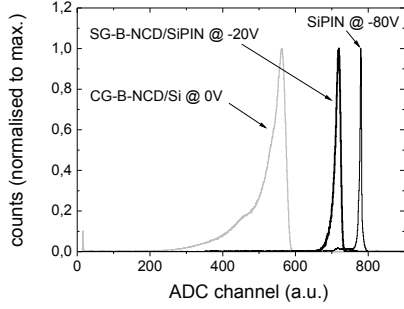
Fig. 6. Comparison of the performance of a CG-BNCD/Si, a SG-BNCD/SiPIN sensors and a commercial SiPIN diode for \alpha -particle detection from an Am-241 spectroscopic-grade solid source. Measurements were performed in vacuum at 10^{-3} mbar, spectra are normalized to the maximum number of counts.
