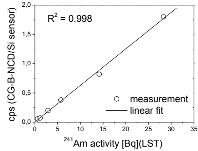
Fig. 8. Integrals of curves derived from Fig 7 vs. total 241 Am solution activity from liquid scintillation technique. This graph shows the perfect linearity of the detection system
