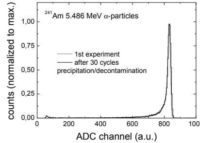
Fig. 10. Spectra of \alpha -particles emitted by ^{241}\text{Am} precipitated on a SG-BNCD/SiPIN sensor: for first experiment (light gray) and after 30 consecutive cycles of electroprecipitation-decontamination. We do not observe any degradation in: precipitation-detection efficiency, position and shape of the spectrum.
