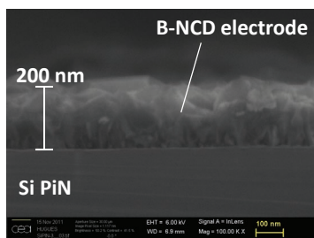
Fig. 1. A SEM photograph showing the cross-section of a 200 nm thick electrochemistry grade BNCD electrode deposited on a SiPiN substrate.
