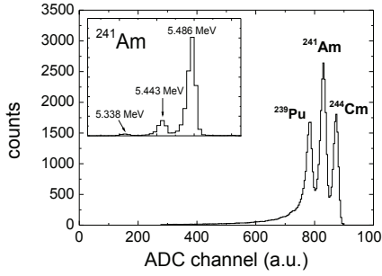
Fig. 9. An \alpha -particle spectrum of mixed nuclide solution (Pu, Am, Cm) measured directly in liquid using electrochemically assisted SG-BNCD/Si sensor. Three peaks corresponding to \alpha -particles emitted by three actinides can be clearly distinguished. The inset shows \alpha -particle spectrum of ^{241}\text{Am} deposited on a BNCD electrode as measured with an external commercial Si PIN detector in vacuum ( 10^{-3} mbar) - Additional two satellites lines are visible around main peak (5.486 MeV) corresponding to alternative decay modes - a proof of spectroscopic grade precipitation of actinides on the sensors
