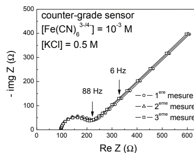
Fig. 2. Electrochemical impedance spectroscopy plot (Nyquist plot) of a CG-BNCD/Si sensor showing the series resistance value (first intercept 100 \Omega ) and the electron transfer resistance (derived from the second intercept 125 \Omega ).
