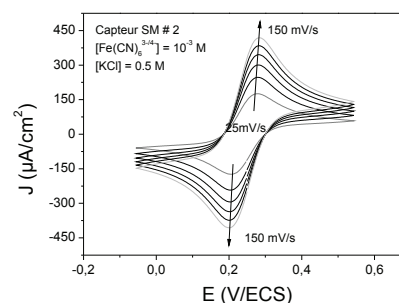
Fig. 3. Cyclic voltammetry curves performed with the CG-BNCD/Si sensor showing the electrochemical activity of the BNCD layer. The measurements are performed using an equimolar solution of potassium ferro-ferricyanide 10^{-3} \text{ M} (outer sphere redox couple) with KCl as supporting electrolyte.
