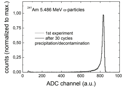
Fig. 10. Spectra of \alpha -particles emitted by ^{241}\text{Am} precipitated on a SG-BNCD/SiPIN sensor: for first experiment (light gray) and after 30 consecutive cycles of electroprecipitation-decontamination. We do not observe any degradation in: precipitation-detection efficiency, position and shape of the spectrum.
