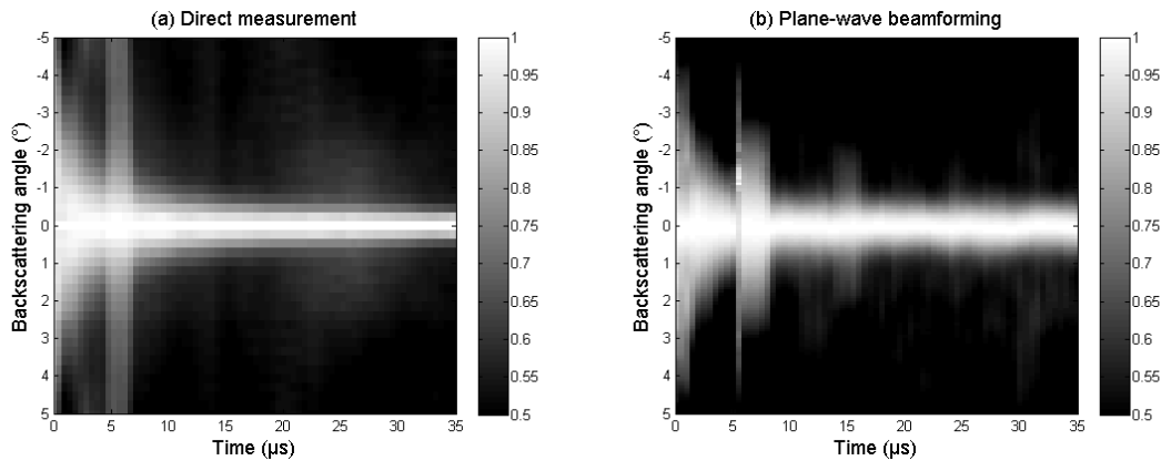
Figure 7. Dynamic backscattered intensity obtained from direct measurement (a) and from plane-wave beamforming technique (b) in the CG sample at 3MHz. At each time step, the intensity is normalised by its maximum along the backscattering angle.
