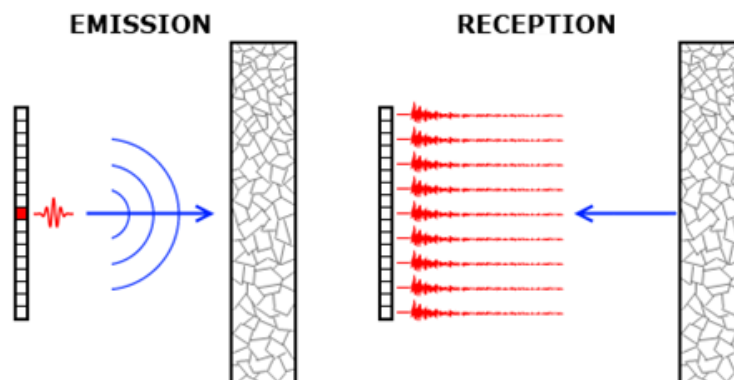
Figure 1. Experimental setup.
