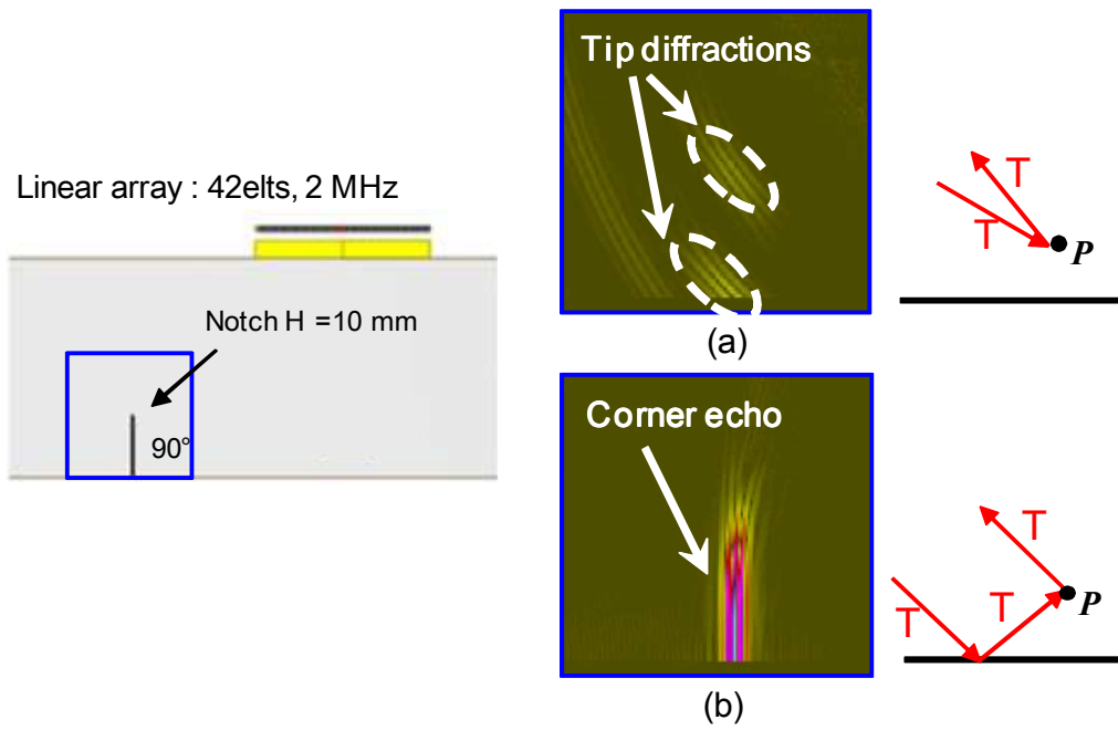
FIGURE 2. Imaging of a vertical breaking notch in a steel block: a) direct TT imaging, b) corner echo TTT imaging.
