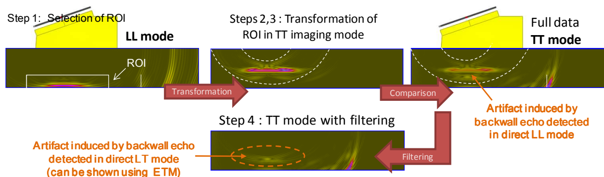
FIGURE 5. Illustration of the principal steps of EMT algorithm.
