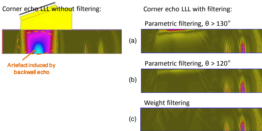
FIGURE 7. Example of application of parametric and weighting filters on a planar component: a) parametric filtering for \hat{\theta} = 130^\circ , b) parametric filtering for \hat{\theta} = 120^\circ , c) weight filtering.
