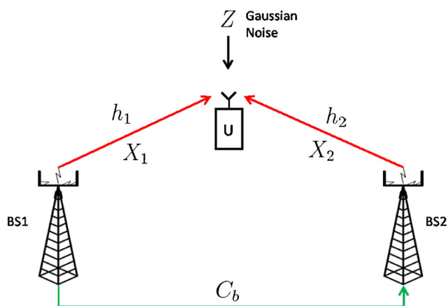
Fig. 1 Downlink base stations cooperation
