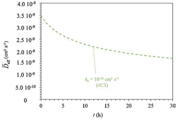
Fig. 7. effective chemical diffusion coefficient as a function of time for Ni-30Cr oxidized at 1173 K calculated by combining Eqs. (3), (4) and (12) assuming a slow cubic grain growth law for case #C3 ( k_h = 10^{-24} \text{ cm}^3 \text{ s}^{-1} ).
