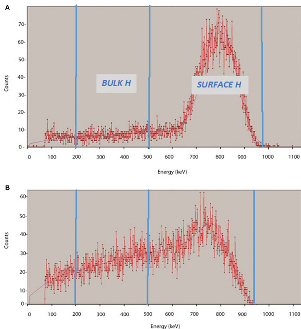
FIGURE 2 | ERDA spectra of two samples with different water concentrations (A) 369b ringwoodite with 0.16 wt% H 2 O and (B) 362 ringwoodite with 1.03 wt% H 2 O. The contribution from surface H is evidenced by the strong peak at high energy. The bulk H content of the crystal is calculated from integration of the signal between 200 and 500 keV.
