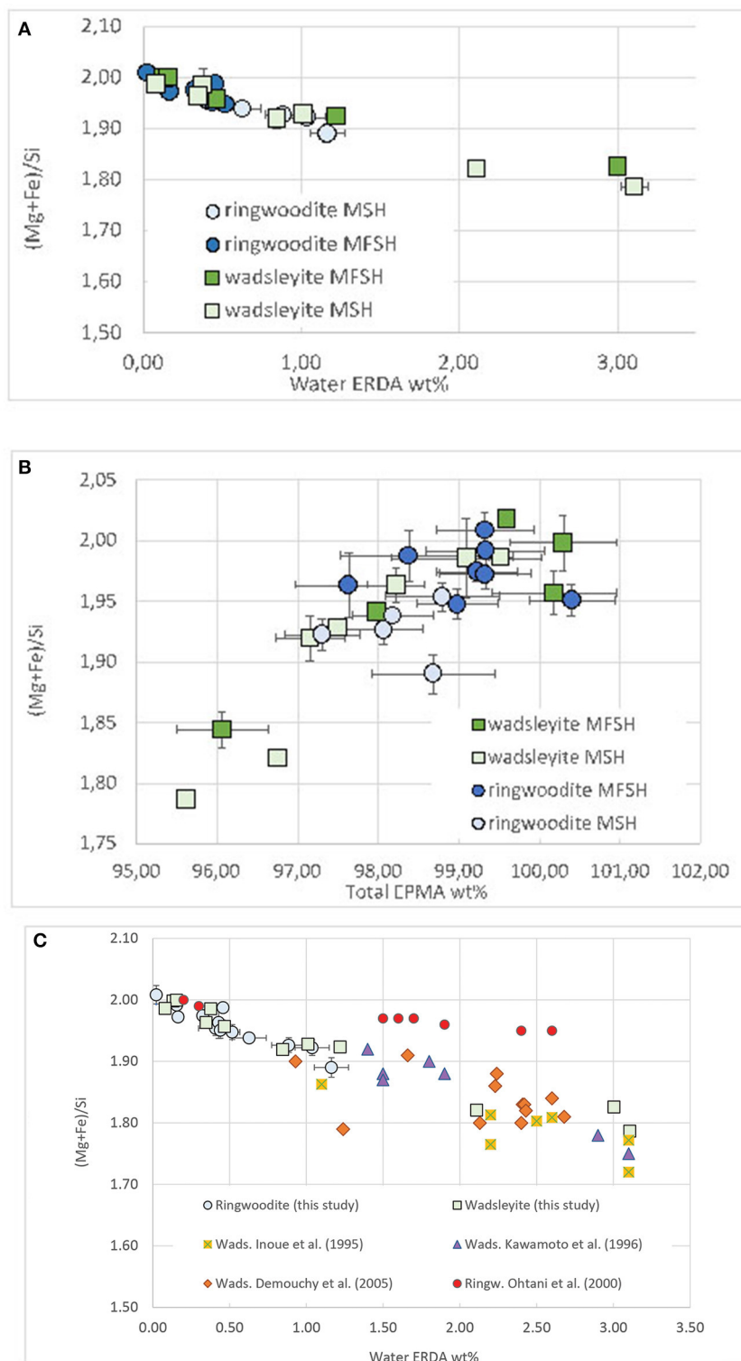
FIGURE 3 | Electron probe micro analyses of wadsleyite and ringwoodite samples from this study in the MSH and MFSH systems. We do not observe any specific effect of the presence of iron. (A) The (\text{Mg}+\text{Fe})/\text{Si} ratio as a function of water content as measured by ERDA. (B) The same ratio as a function of EPMA weight totals. This plot evidences the lack of precision of EPMA analysis totals to measure quantitatively water contents. (C) (\text{Mg}+\text{Fe})/\text{Si} ratio compiled for all systematic studies, showing a satisfying agreement between SIMS and ERDA data for wadsleyite, but not for ringwoodite at high water contents. All previous studies were focused on wadsleyite samples, except that of Ohtani et al. (2000) focusing on ringwoodite samples.
