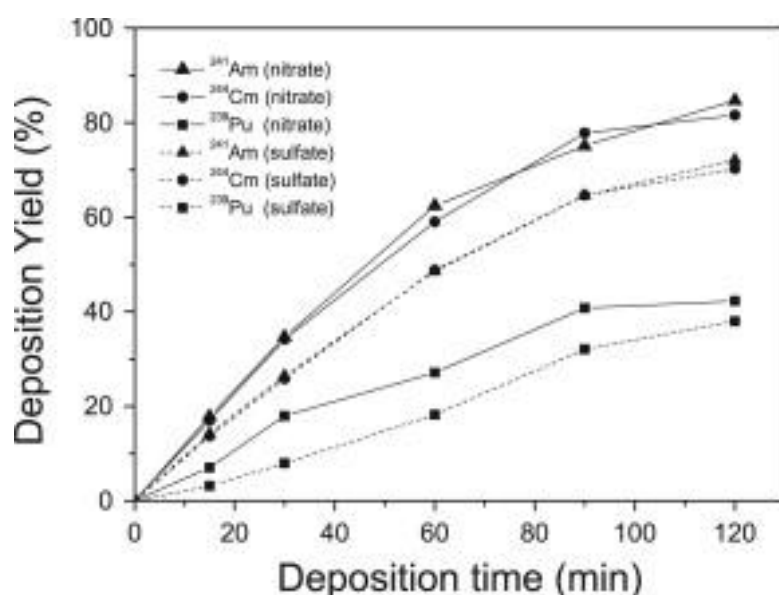
Fig. 3. Deposition kinetics of 241 Am (5.96 Bq), 239 Pu (5.13 Bq) and 244 Cm (4.40 Bq) on B-NCD/Si substrates, [Na 2 SO 4 ]=0.3 M at pH 3.5 with J_c = -5 mA/cm 2 , [NaNO 3 ]=0.3 M at pH 3 with J_c = -2.5 mA/cm 2 , electrolyte: 18 ml, cathode surface area: 1.2 cm 2 , and stirring rate: 10 3 rpm.
