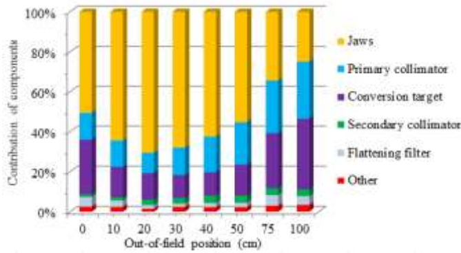
Fig. 10. Contribution of the accelerator components in each position of the photon neutron profile for 20 MV photons.
