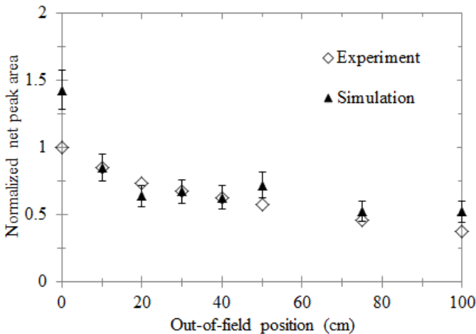
Fig. 12. Comparison between simulated and measured photon neutron profiles for 20 MV photons, simulation model corrected, activation detector containing a foil of vanadium.
