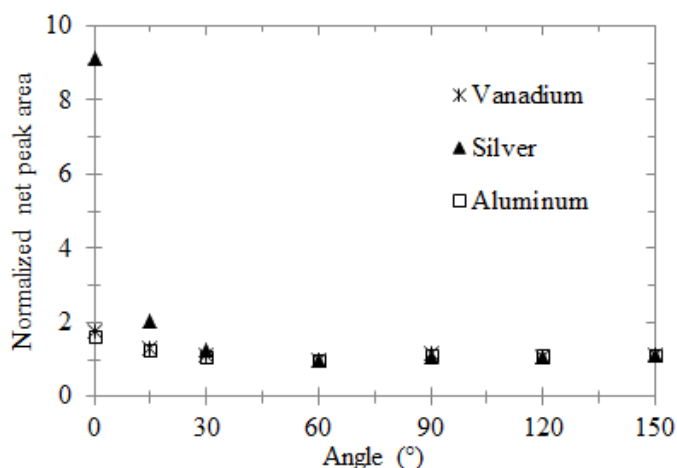
Fig. 4. Angular distribution of the photoneutron flux emitted by a tantalum target irradiated by 17 MeV electrons, activation detector containing a foil of vanadium, silver, or aluminum.
