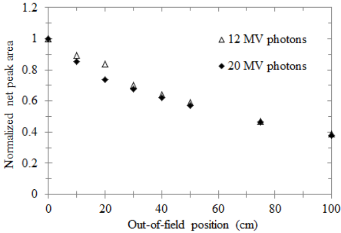
Fig. 8. Photoneutron profiles measured at the Saturne 43F medical accelerator with an activation detector containing a foil of vanadium for 12 MV or 20 MV photons.
