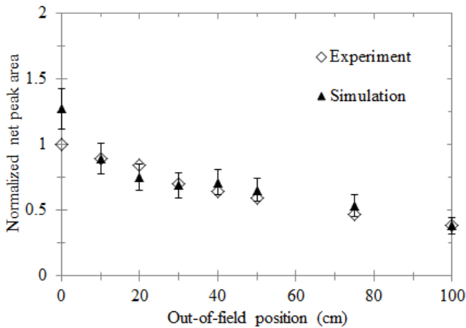
Fig. 11. Comparison between simulated and measured photon neutron profiles for 12 MV photons, simulation model corrected, activation detector containing a foil of vanadium.
