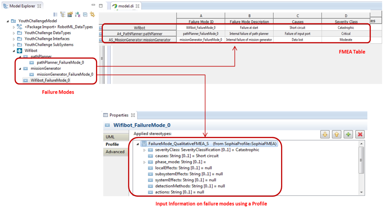
Figure 4. Sophia-FMEA modeler
