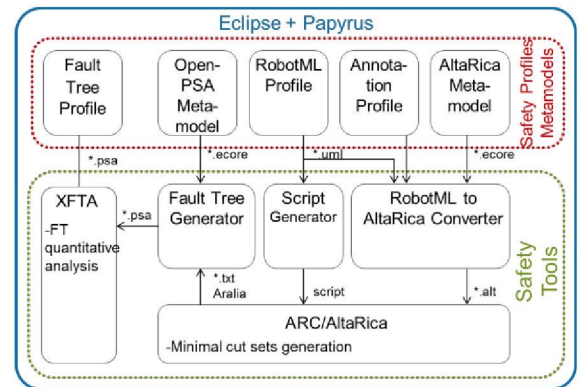
Figure 3. The architecture of the framework
