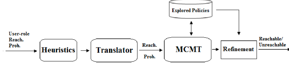
Fig. 2. ASASPXL architecture
