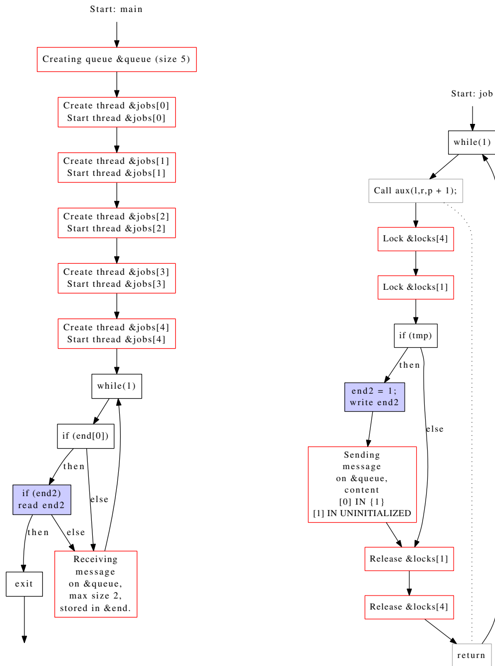
Fig. 22. Concurrent control-graphs for threads main and &jobs [0]
