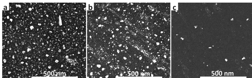
FIGURE 3. SEM pictures of diamond nanoparticles deposited on a PDDAC-coated Cr substrate using (a) ND-30 solution over 1 min, (b) ND-30 solution over 5 s, and (c) ND-30 solution diluted c/10 over 5 s.
