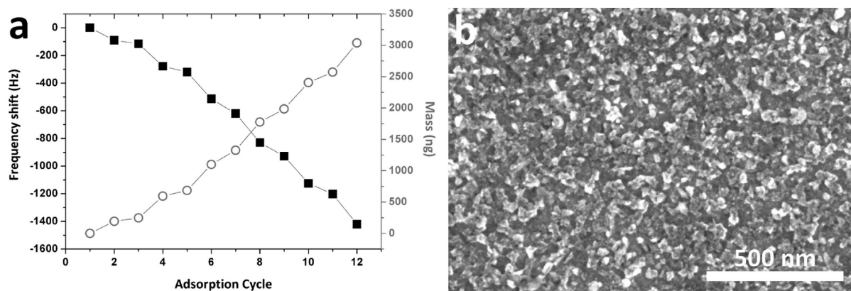
FIGURE 5. (a) QCM measurements, giving the frequency shift and calculated mass adsorbed according to each deposited layer of ND-30 and PDDAC polymer. The first adsorption corresponds to deposition of PDDAC. (b) SEM picture of six ND-30/PDDAC layers.
