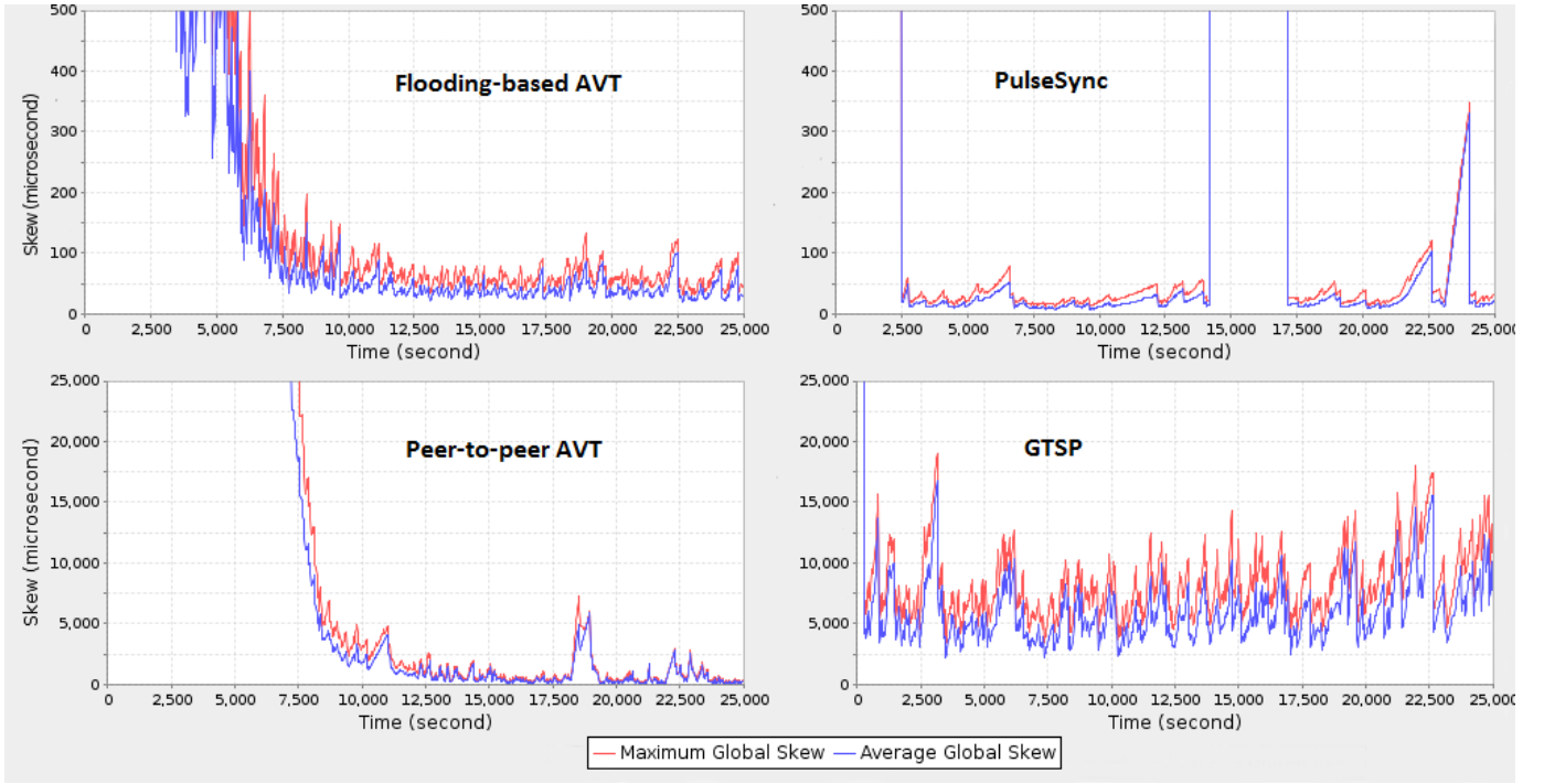
Fig. 3. Global synchronization errors observed in our simulations.
