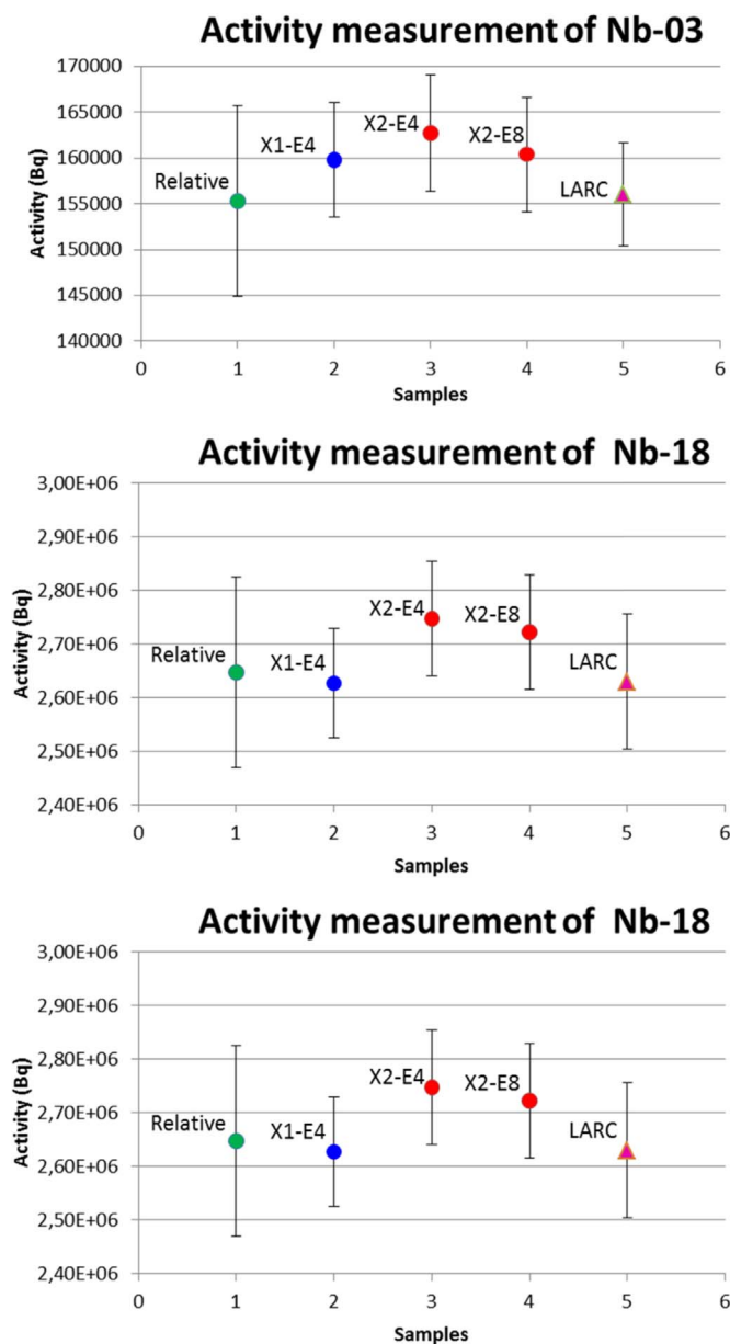
Fig. 5. Comparison of niobium activity measurements ( k = 1 ) using 3 different techniques.
