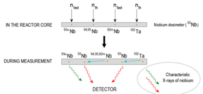
Fig. 4. Self-fluorescence in a niobium dosimeter.
