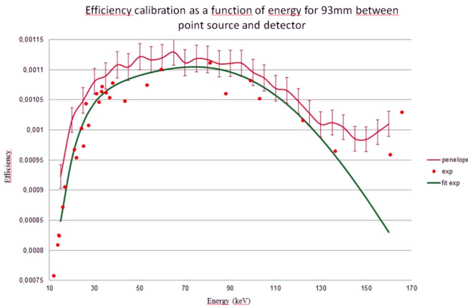
Fig. 2. Comparison between simulation and experimental efficiency of channel \times 2 -E8.
