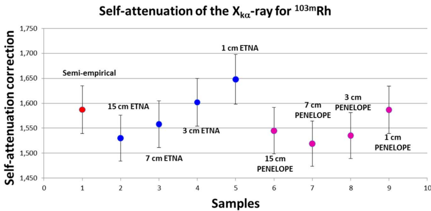
Fig. 3. Self-attenuation of the X_{k\alpha} -ray line of ^{103m}\text{Rh} ( k = 1 ) in rhodium 50 \mu\text{m} thickness sample as a function of the measuring distance between sample and detector (cm).
