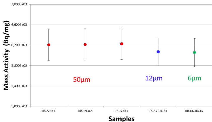
^{103\text{m}}\text{Rh} activity measurement for different thicknesses at the same location
