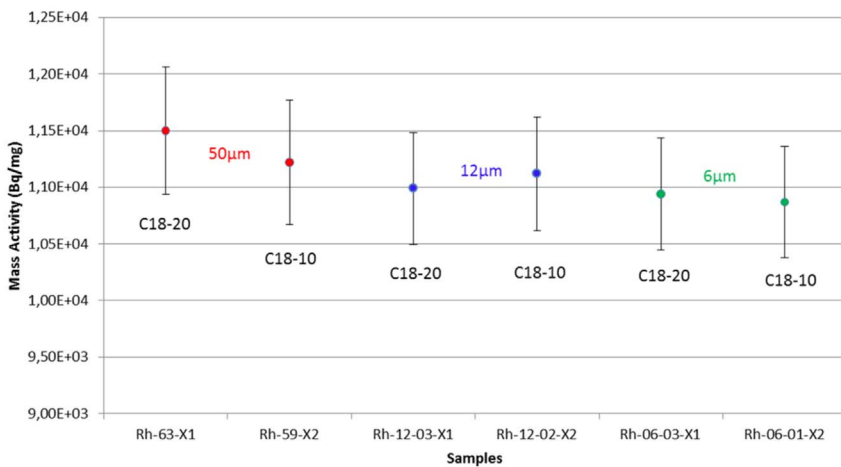
^{103\text{m}}\text{Rh} activity measurement for different thicknesses at the same location
