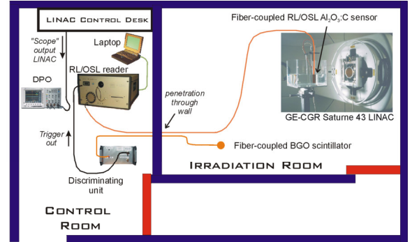
Fig 2. Experimental set-up. The RL/OSL sensor is immersed within a water phantom in reference conditions [1]. A fiber-coupled BGO scintillator (placed next to the LINAC) provides light pulses in phase with LINAC pulses. The discriminating unit provides a TTL signal that serves to trigger the logic gate inserted within the RL-OSL reader to wipe out the stem effect.
