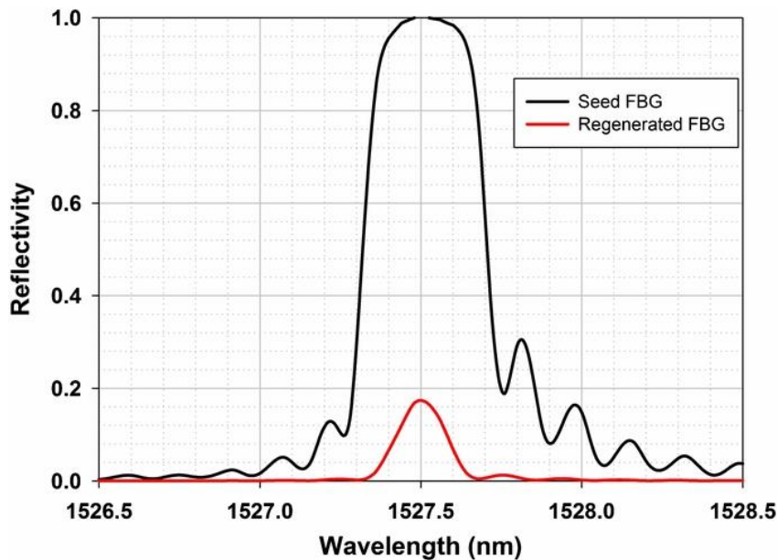
Figure 4. Spectrum of a seed FBG and that of the corresponding regenerated FBG (both spectra acquired at room temperature).
