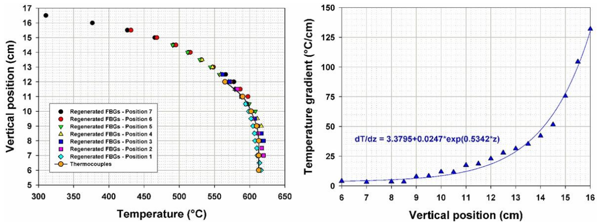
Figure 8. Temperature profile and gradient of the tubular furnace reconstructed by an array of ten multiplexed regenerated FBGs.
