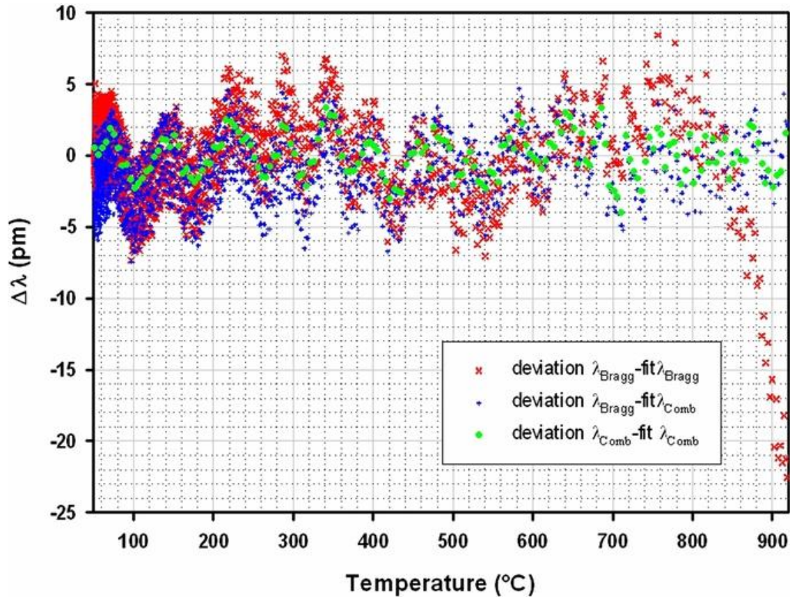
Figure 7. Deviations between the experimental Bragg wavelengths with regard to a fifth-order polynomial fitting processed on averaged (blue point, subset averaged every 5 °C) and non-averaged (red point) data. The green points stand for the error between the averaged data and the polynomial fit computed thereon.
