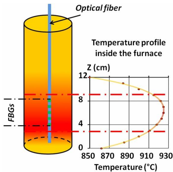
Figure 3. Temperature gradient within the heating zone used for the regeneration process.
