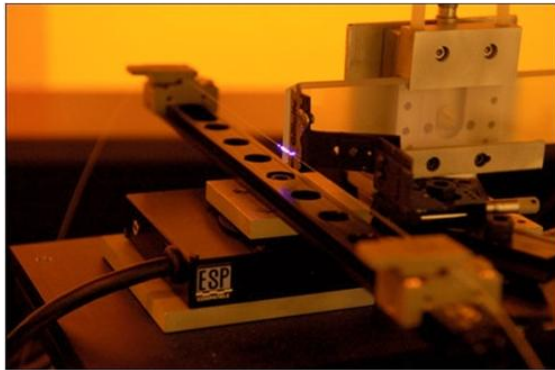
Lloyd interferometric setup
