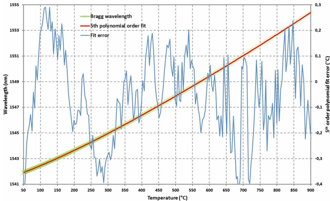
Figure 6. Fifth-order polynomial fit of the Bragg wavelength over a range of 850 °C.
