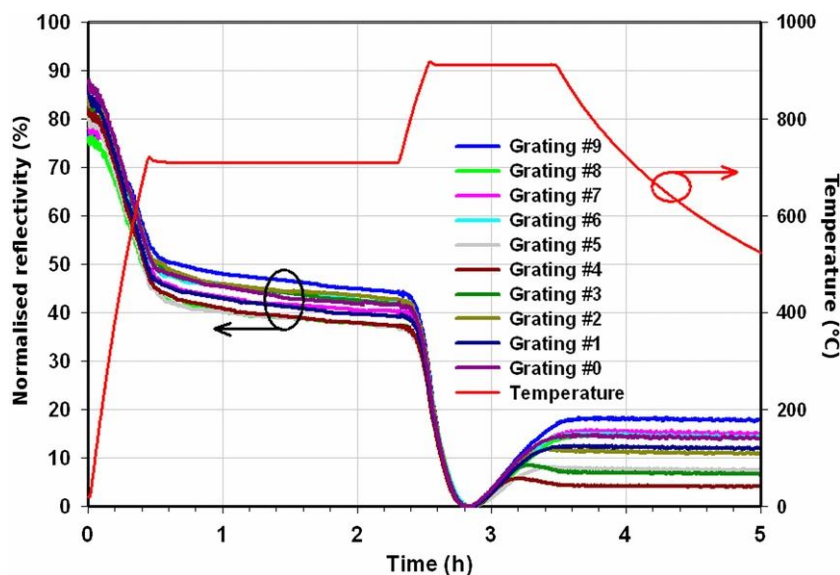
Figure 5. Evolution of the reflection signal from the ten multiplexed seed FBGs regenerated simultaneously.
