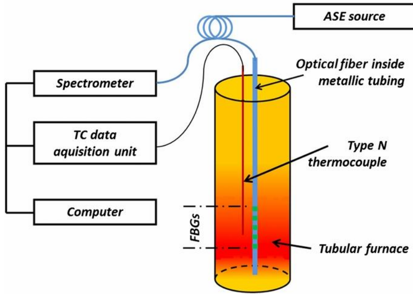
Figure 2. Annealing setup for FBG regeneration.
