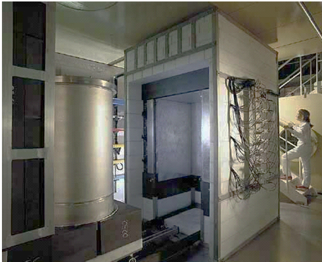
Fig. 29. CHICADE's graphite neutron measurement cell for 200 L drums SYMETRIC, including 99 ^3\text{He} proportional counters with charge preamplifiers connected to an electronics counting coincidences between spontaneous fission neutrons (passive mode) or prompt and delayed fission neutrons induced by the use of a 2 \cdot 10^9 \text{ n.s}^{-1} high flux neutron generator (active neutron interrogation).
