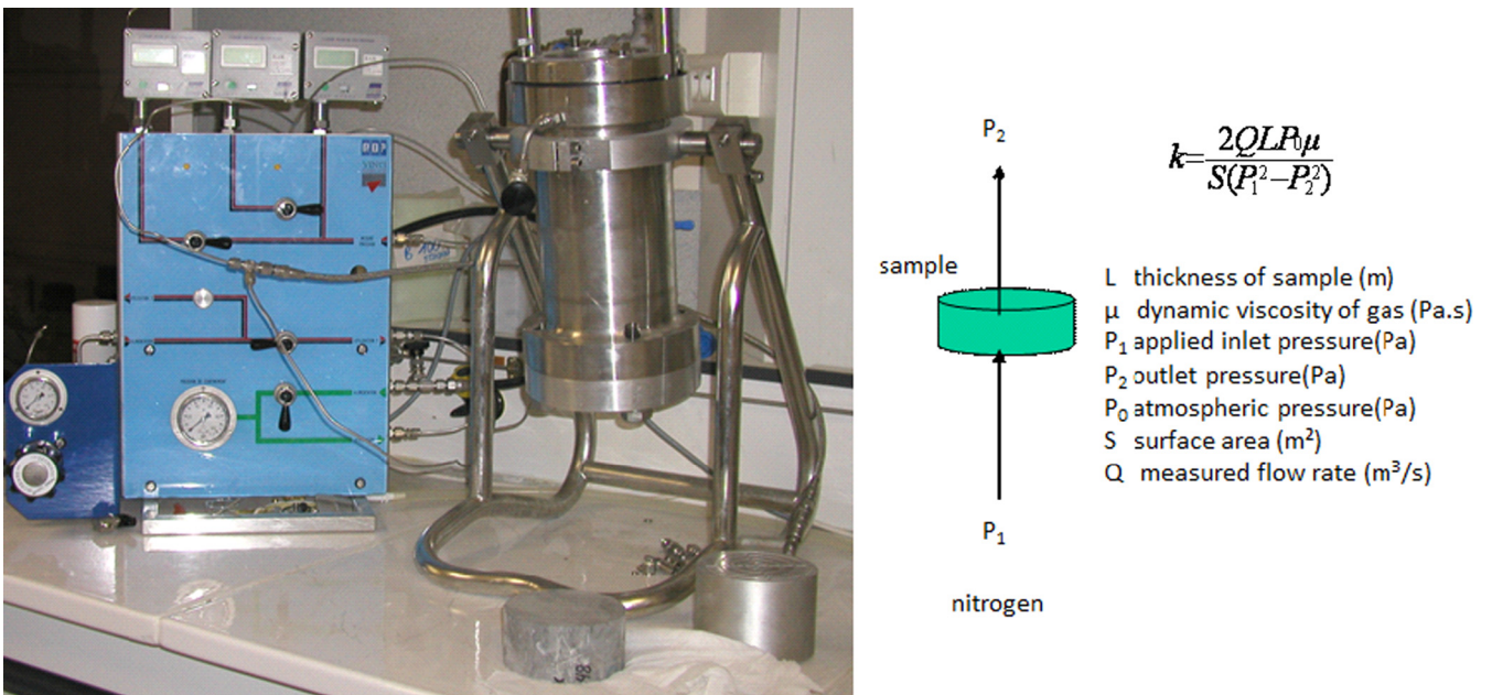
Fig. 25. Measurement of gas permeability. The concrete test specimen is placed in the cell and leak tightness on the sides of the test specimen is ensured by a pressure of 60 bars. Afterwards, a pressure of 2 bars is applied to the bottom side of the test specimen and the flowrate crossing through the specimen is measured.
