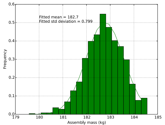
Fig. 4. Dispersion of the assembly mass due to the uncertainties on the helium production.
