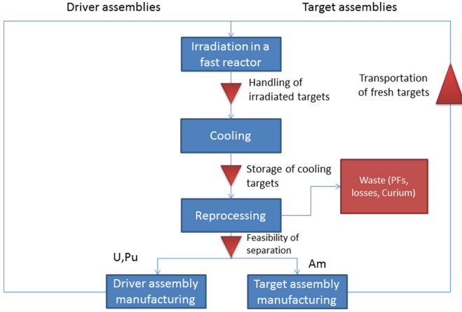
Fig. 1. Fuel cycle considered for this study.
