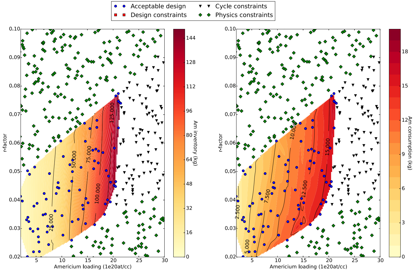
Fig. 9. Americium inventory and consumption for one blanket assembly for a 3600 MWth oxide core conditions. A 7.5 kW decay heat limit was considered here. All the parameters of the assembly design model were used as free parameters. Zirconium hydride was used as moderating material.
