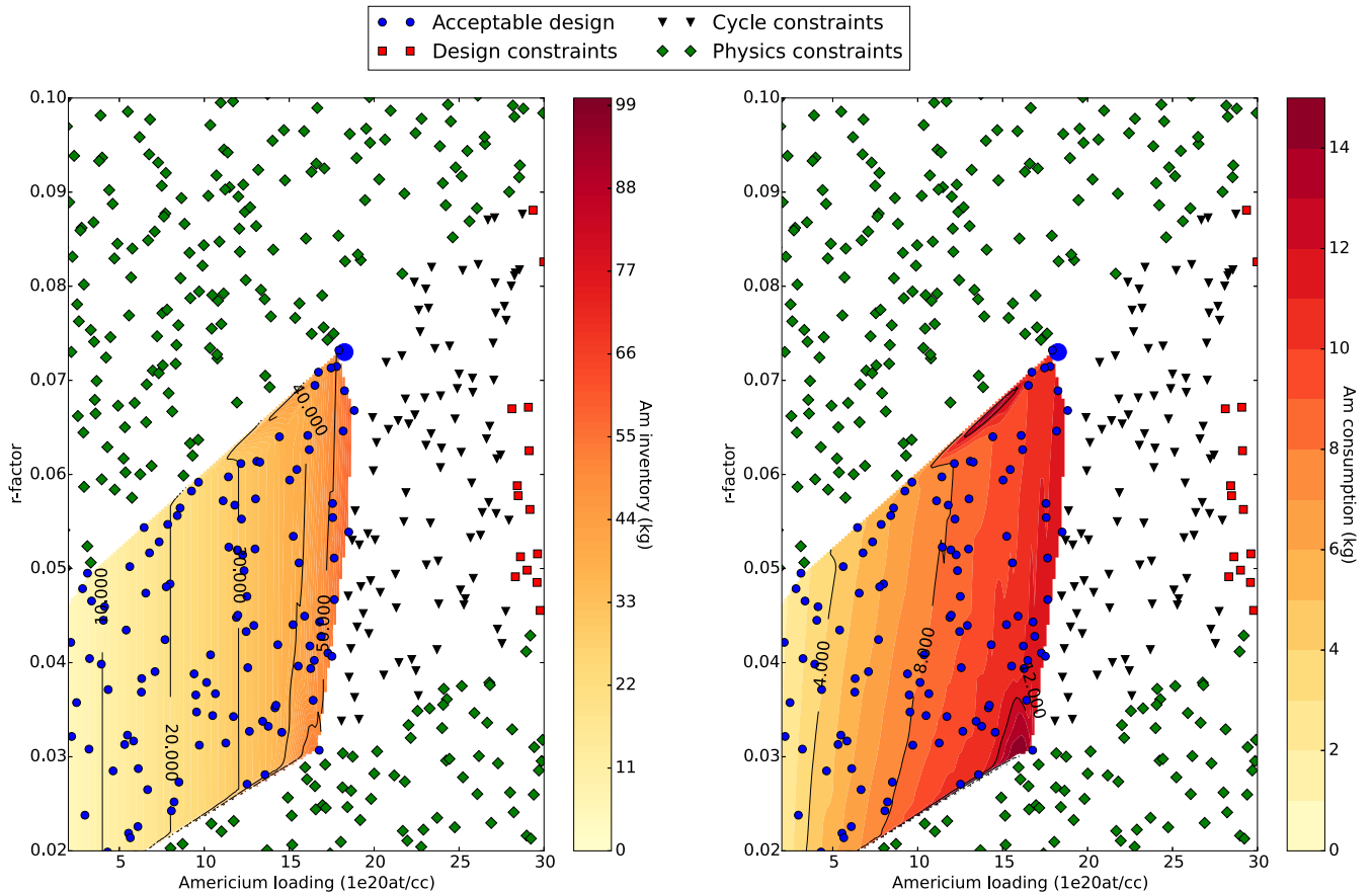
Fig. 8. Am inventory and consumption for one blanket assembly for a 3600 MW core with a 7.5 kW cooling limit pellet diameter and plenum height optimization. The larger blue circle corresponds to SFR V2b situation.
