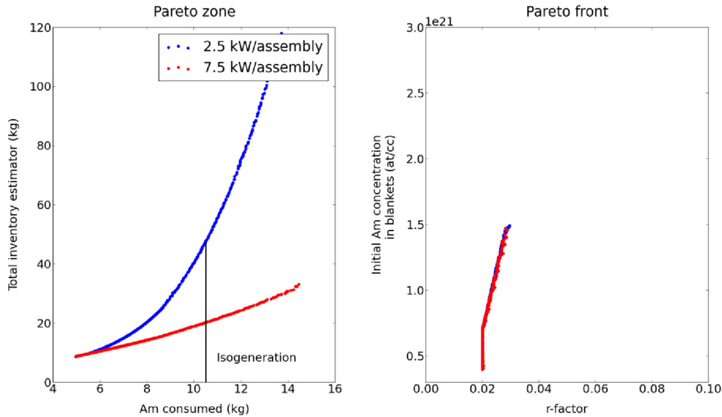
Fig. 10. Pareto front and zone with regards to consumption and Am inventory in the fuel cycle for an oxide core. The irradiation time was maximized at 6000 EFPD and the assembly design was optimized with regards to the pellet diameter and gas plenum expansion height.
