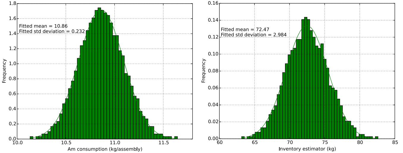
Fig. 5. Dispersion of the Am inventory and consumption per assembly due to the uncertainty on helium production.
