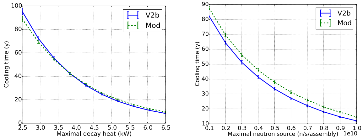
Fig. 3. Evaluation of the errors due to the meta-models approximation on the cooling time for two reference cases.
