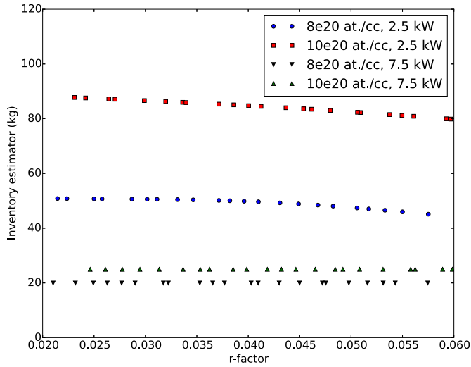
Fig. 7. Evolution of the inventory estimator with regards to the r -factor for various washing limits and Am loadings. Only the pellet diameter was used as an optimization parameter for the assembly design.
