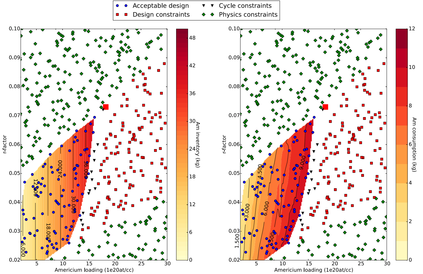
Fig. 6. Am inventory and consumption for one blanket assembly for a 3600 MW core with a 7.5 kW cooling limit pellet diameter optimization. The large red square corresponds to SFR V2b situation.
