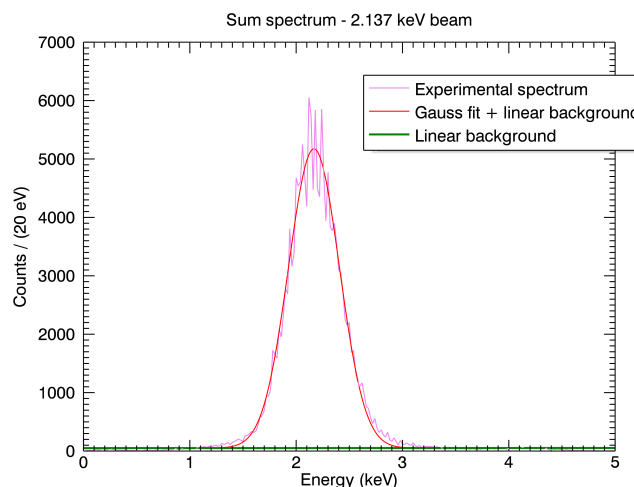
Fig. 6. Example of sum-spectrum obtained with the 2.137 keV beam. The photopeak can be fitted by a Gaussian function.
