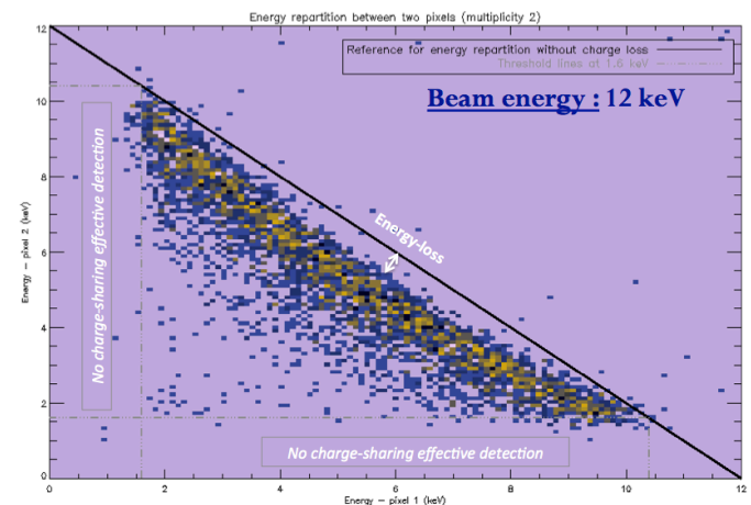
Fig. 9. Energy repartition between two neighbor pixels touched simultaneously, with a 12 keV beam.
