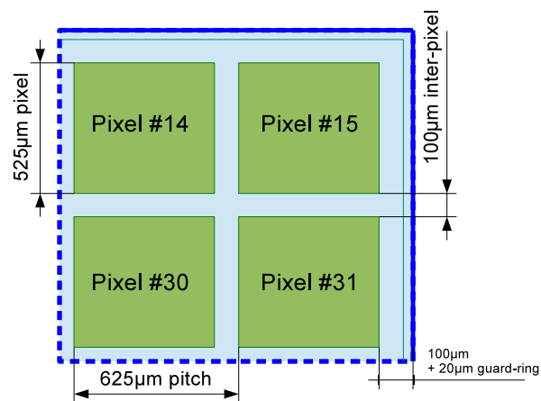
Fig. 2. Scheme of the right top corner of the subdivided anode with pixel size and inter-pixel zone, plus the 20 μm guard ring.
