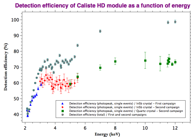
Fig. 7. Detection efficiency measured for single and multiple events, between 2.137 and 12 keV. Two series of runs were represented, for different monochromators used in SOLEX facility.
