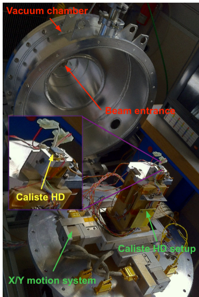
Fig. 3. Caliste HD characterization setup (opened).
