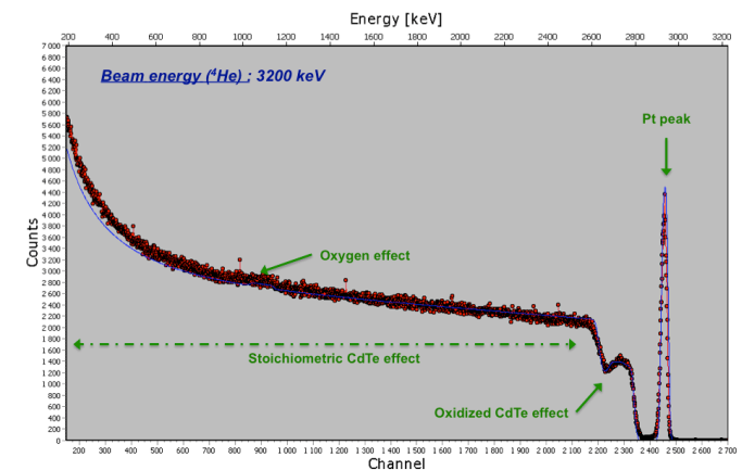
Fig. 11. RBS spectrum obtained with a ^4He beam of 3.2 MeV. Experimental points are in red, and the simulated curve is blue.
