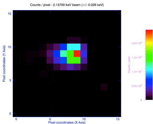
Fig. 5. Image obtained with a 2.137 keV spot. With a pitch of 625 micrometers, we can estimate the spot size to a maximum of 3.75 mm (X axis) and 2.5 mm (Y axis). The color scale represents the count rate of each pixel.
