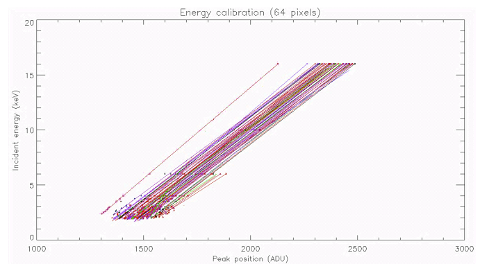
Fig. 4. Incident energy (keV) as a function of peak amplitude (ADU), for the 64 most active pixels – First campaign.
