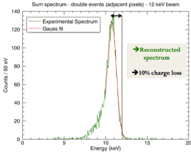
Fig. 10. Reconstructed spectrum for double events, with a 12 keV beam.
