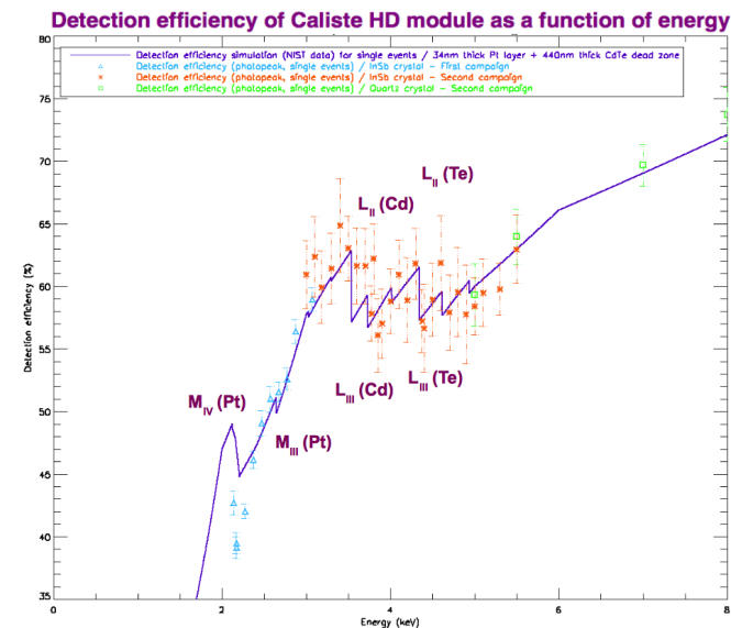
Fig. 8. Detection efficiency measured and simulated for single events, between 2.137 and 8 keV. Two series of runs were represented, for different monochromators used in SOLEX facility. Characteristic X-rays absorption edges are marked.
