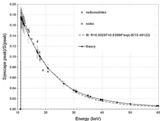
Figure 4. Escape to PE peak area ratio of the germanium detector (SOLEX and radionuclides' data).
