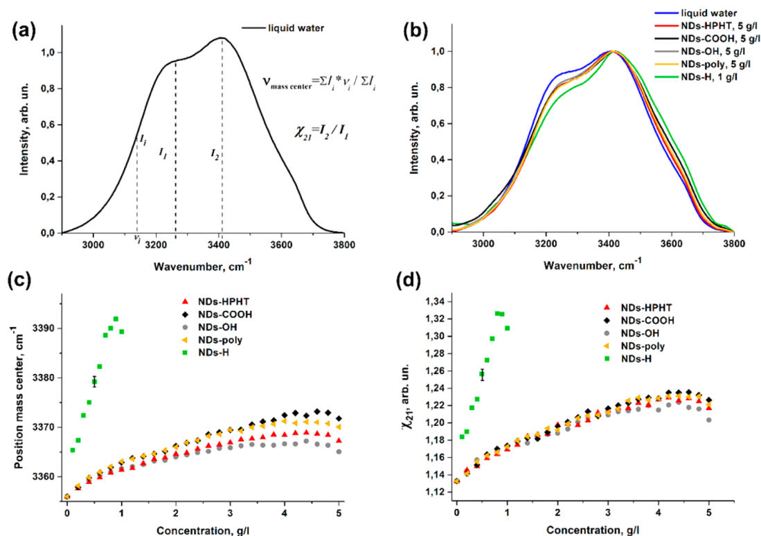
Figure 3. (a) Illustration of calculation of the position of mass center ( \nu_{\text{mc}} ) and parameter \chi_{21} of water Raman OH stretching bands. (b) Raman OH stretching bands of aqueous dispersions of NDs. The spectra were normalized to the maximum I_2 of the stretching bands. Dependence of \nu_{\text{mc}} (c) and \chi_{21} (d) in NDs aqueous dispersions with respect to the NDs concentration.
