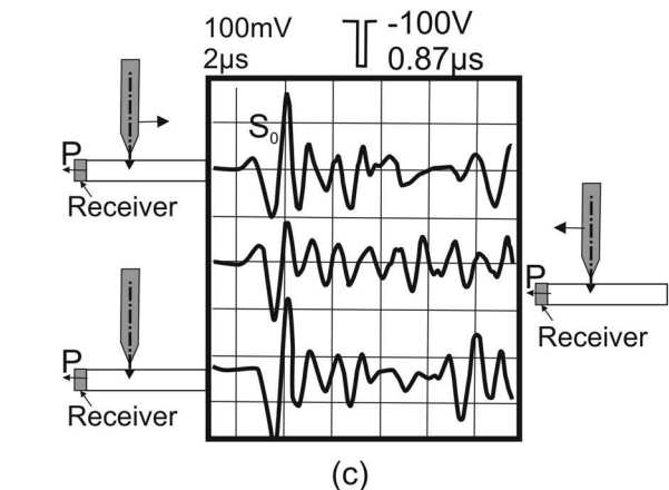
Fig. 8. S_0 tangential component dependency on (a) rotation, (b) inclination, and (c) sliding of the stylus for an axial vibration of the tip.
