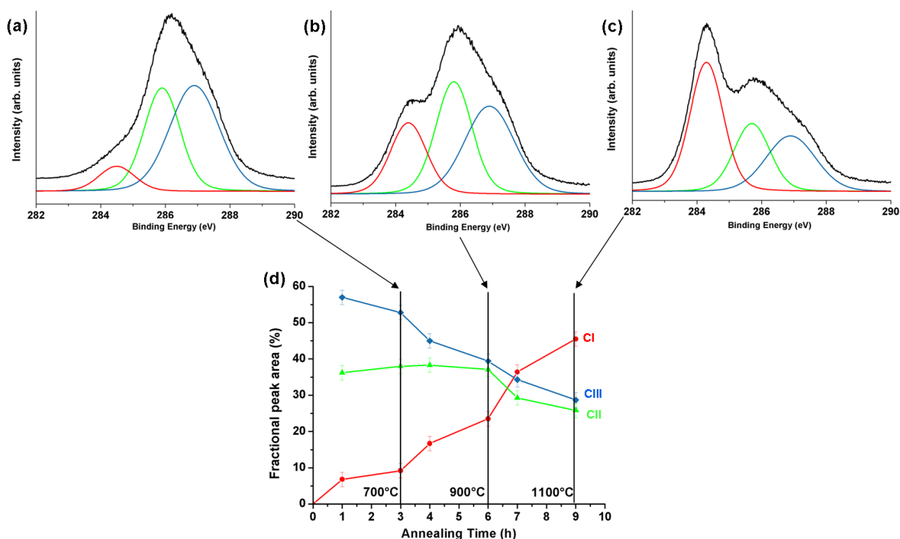
Figure 15 Evolution of C1s core level for different annealing temperatures and annealing times, CI, CII and CIII correspond to sp^2 carbon, sp^3 carbon and defects, respectively [78].
