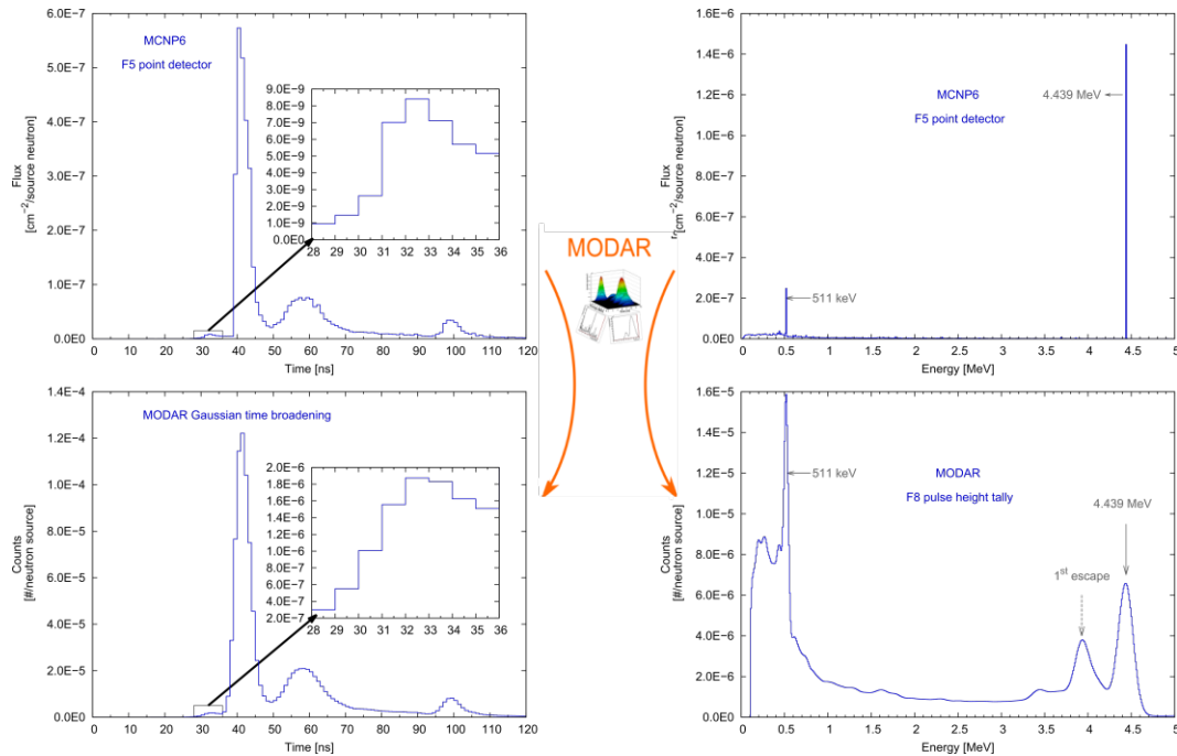
Fig. 4: Conversion of the photon flux reaching a 5'' x 5'' x 10'' NaI detector into TOF (left) and gamma (right) spectra using MODAR, in case of a carbon target.
