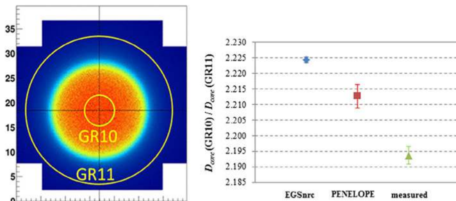
Fig. A1. Left hand side, representation of the core diameters for the GR11 and GR10 calorimeters (yellow circles) in a 2 cm diameter beam (measured with EBT3 films) and right hand side, D_{core}(GR10)/D_{core}(GR11) ratios measured and calculated with EGSnrc and PENELOPE (error bars are type A uncertainties at one standard deviation).
