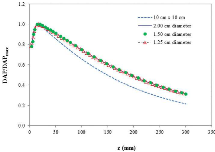
Fig. 4. Normalized depth ionization curves (SSD 100 cm) measured with a PTW 34070 ionization chamber with collecting electrode diameter of 8.16 cm at 6 MV for the reference field size (10 cm × 10 cm) and three stereotactic beams with diameter 2.00 cm, 1.50 cm and 1.25 cm at the phantom surface.
