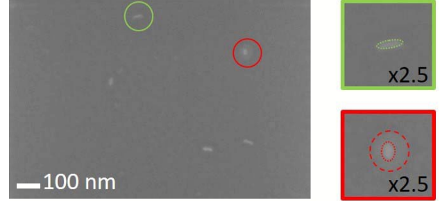
Fig. 6 SEM characterization of single GNRs in the absence (green circle) or after “over-illumination” (red circle). A pulse energy density of 2.5 mJ.cm -2 was used with an incident polarization along the longitudinal axis of the GNR and at its longitudinal plasmon resonance wavelength. In the SEM images, dotted lines delineate the GNR from an additional halo observed following high power excitation. The dashed red line delineates a halo around the GNR. The GNR after illumination presents an aspect ratio of around 2. The GNR is clearly shorter than the one illuminated with a 125 \mu\text{J.cm}^{-2} pulse energy density as shown in Fig. 3.
