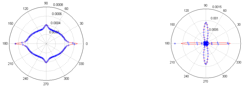
Fig. 1. Out of plane displacement of the A0 mode at a distance of 100mm at the frequency of 300 kHz of an excitation by a circular source (left) or by a square source (right) calculate by a full integration (red line) and an integration along energy direction (blue cross) .
