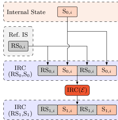
Figure 7: IRC on stream ciphers - initialization step
