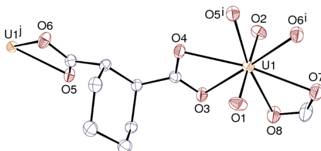
Figure 2. View of compound 2 . Displacement ellipsoids are drawn at the 20% probability level. Counterions and hydrogen atoms are omitted. Symmetry codes: i = 1 - x, y + 1/2, 2 - z ; j = 1 - x, y - 1/2, 2 - z . The packing is similar to that in 1 .
