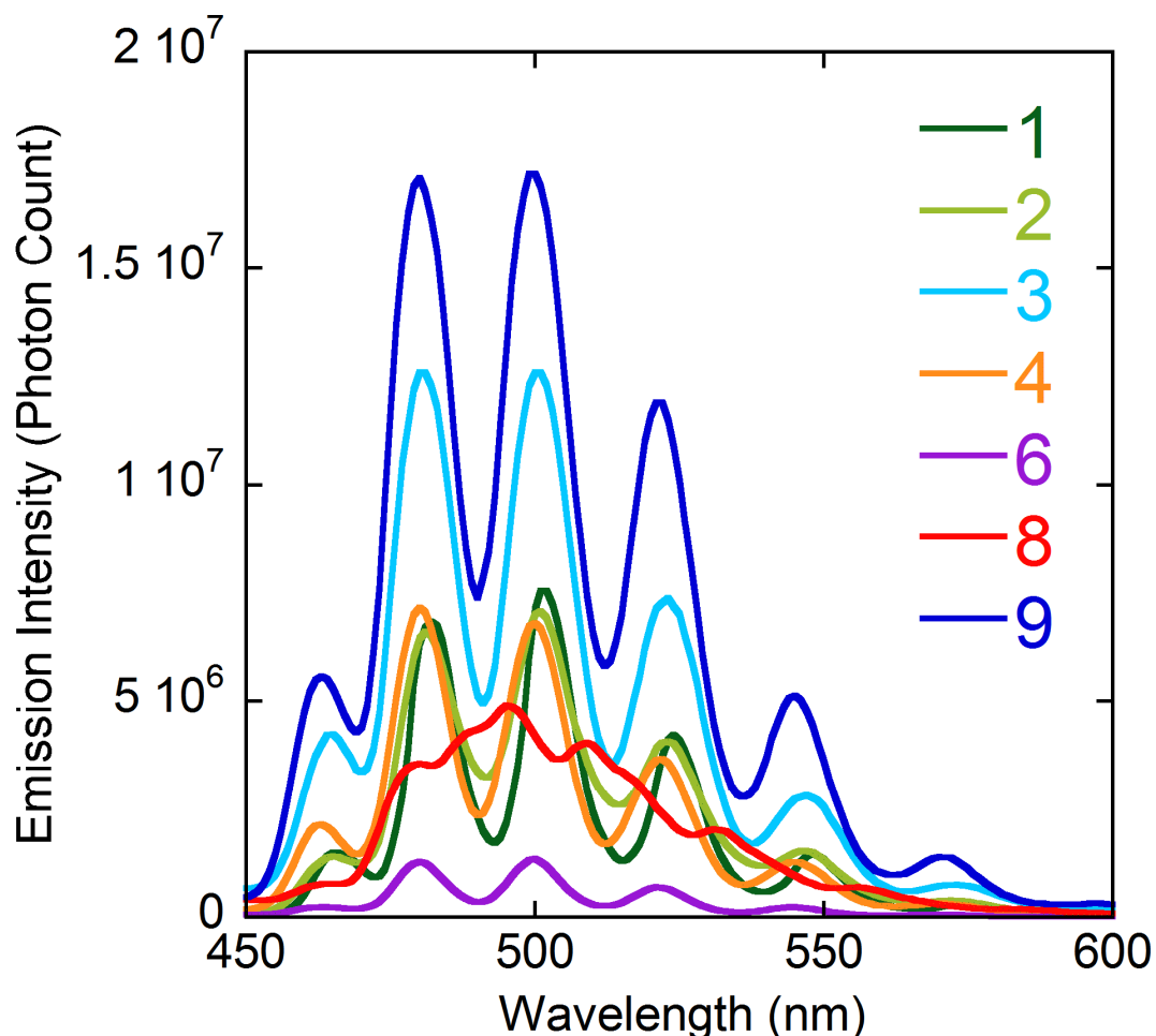
Figure 11. Emission spectra of compounds 1–4 , 6 , 8 and 9 in the solid state, under excitation at a wavelength of 420 nm.
