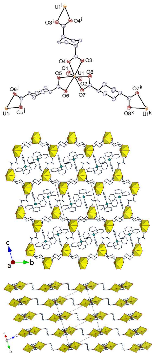
Figure 7. Top: View of compound 6 . Displacement ellipsoids are drawn at the 50% probability level. Counterions, solvent molecules and hydrogen atoms are omitted. Symmetry codes: i = 1 - x, -y, 1 - z ; j = 2 - x, 1 - y, 2 - z ; k = -x, -y, 2 - z . Middle: View of the uranyl-based 2D network and the counterions. Bottom: Packing of the sheets with counterions and solvent molecules omitted.
