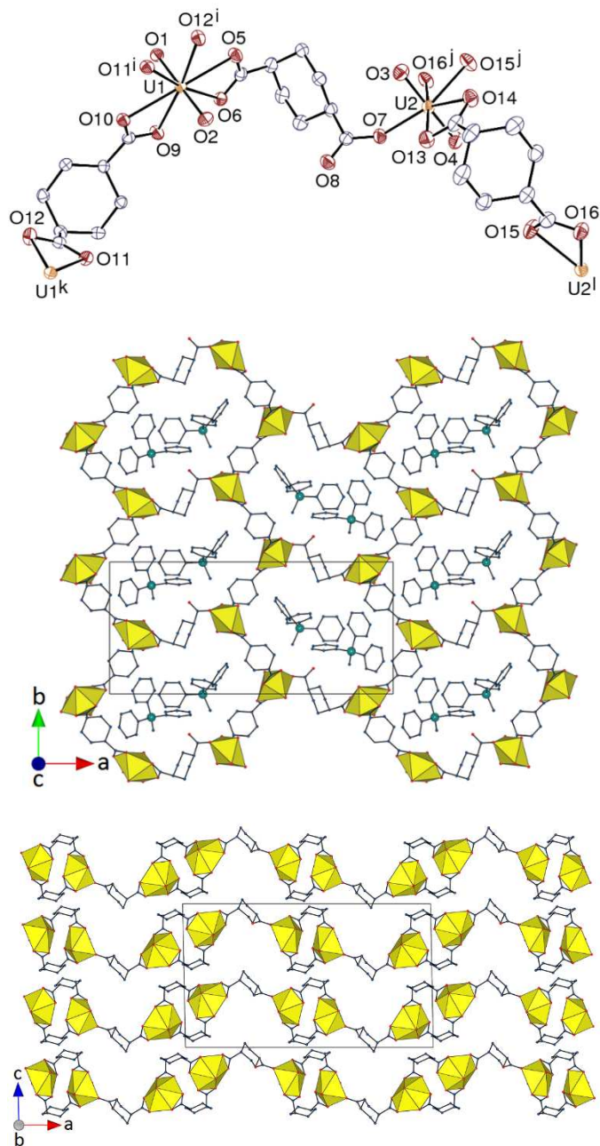
Figure 9. Top: View of compound 8 . Displacement ellipsoids are drawn at the 50% probability level. Counterions, solvent molecules and hydrogen atoms are omitted. Symmetry codes: i = -x, y - 1/2, 1/2 - z ; j = 1 - x, y - 1/2, 1/2 - z ; k = -x, y + 1/2, 1/2 - z ; l = 1 - x, y + 1/2, 1/2 - z . Middle: View of the uranyl-based 2D network and the counterions. Bottom: Packing of the sheets with counterions and solvent molecules omitted.
