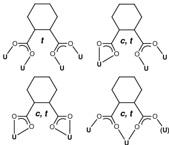
Scheme 1. Coordination modes of c - and t -1,2-chdc 2- in uranyl ion complexes.
