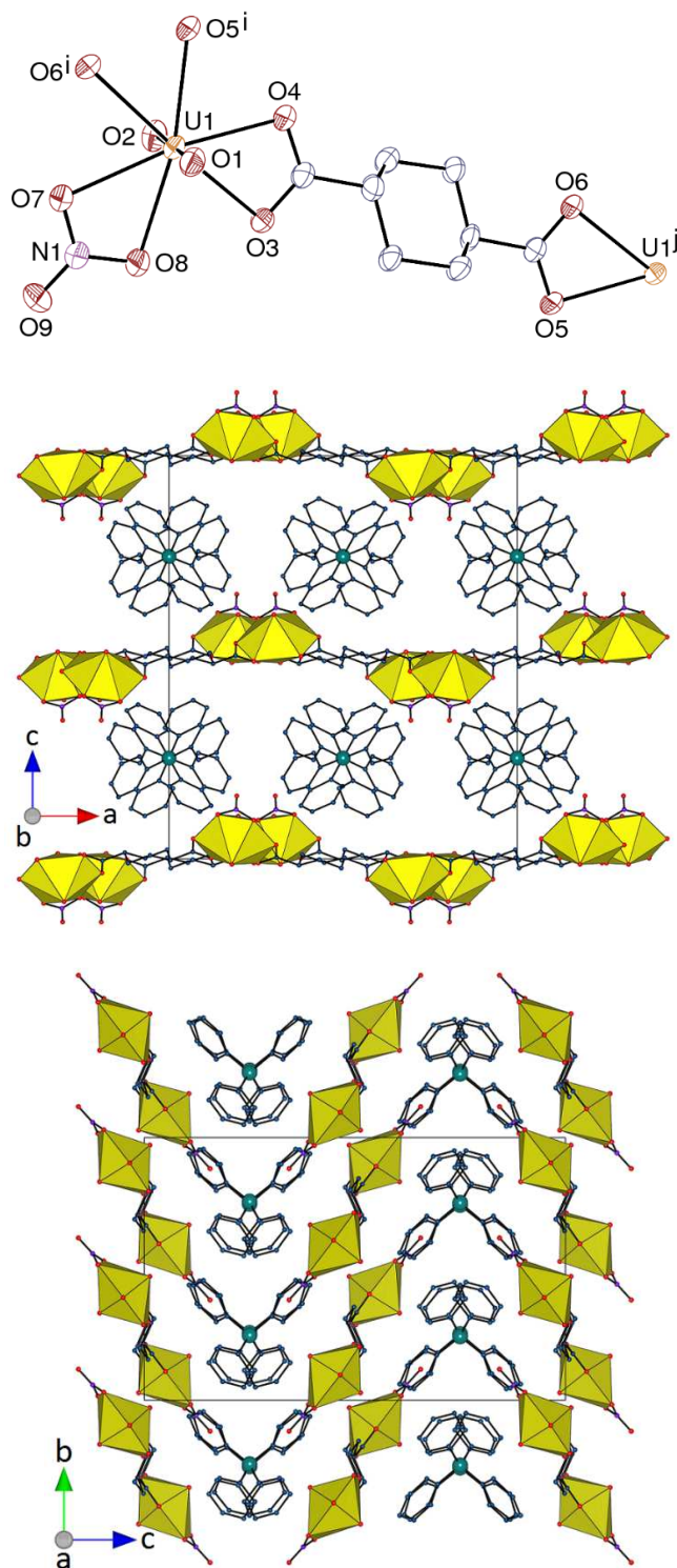
Figure 5. Top: View of compound 4 . Displacement ellipsoids are drawn at the 50% probability level. Counterions, solvent molecules and hydrogen atoms are omitted. Symmetry codes: i = x - 1/2, 1/2 - y, 1 - z ; j = x + 1/2, 1/2 - y, 1 - z . Middle and bottom: Packing with chains viewed side-on or end-on, respectively, and solvent molecules and hydrogen atoms omitted.
