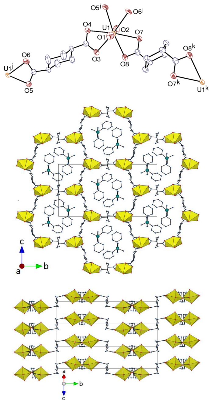
Figure 8. Top: View of compound 7 . Displacement ellipsoids are drawn at the 50% probability level. Counterions, solvent molecules and hydrogen atoms are omitted. Symmetry codes: i = x + 1, 3/2 - y, z + 1/2 ; j = x - 1, 3/2 - y, z - 1/2 ; k = 2 - x, 2 - y, 1 - z . Middle: View of the uranyl-based 2D network and the counterions. Bottom: Packing of the sheets with counterions and solvent molecules omitted.
