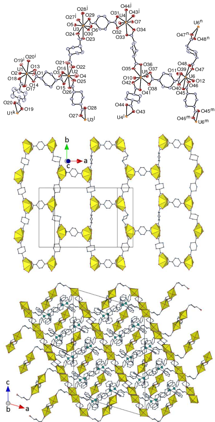
Figure 10. Top: View of compound 9 . Displacement ellipsoids are drawn at the 40% probability level. Counterions, solvent molecules and hydrogen atoms are omitted. Symmetry codes: i = -x - 1/2, y - 1/2, 1/2 - z ; j = x, y - 1, z ; k = -x - 1/2, y + 1/2, 1/2 - z ; l = x, y + 1, z ; m = 2 - x, 2 - y, 1 - z ; n = 2 - x, 1 - y, 1 - z . Middle: View of the uranyl-based 2D network. Bottom: Packing with sheets viewed edge-on and solvent molecules omitted.
