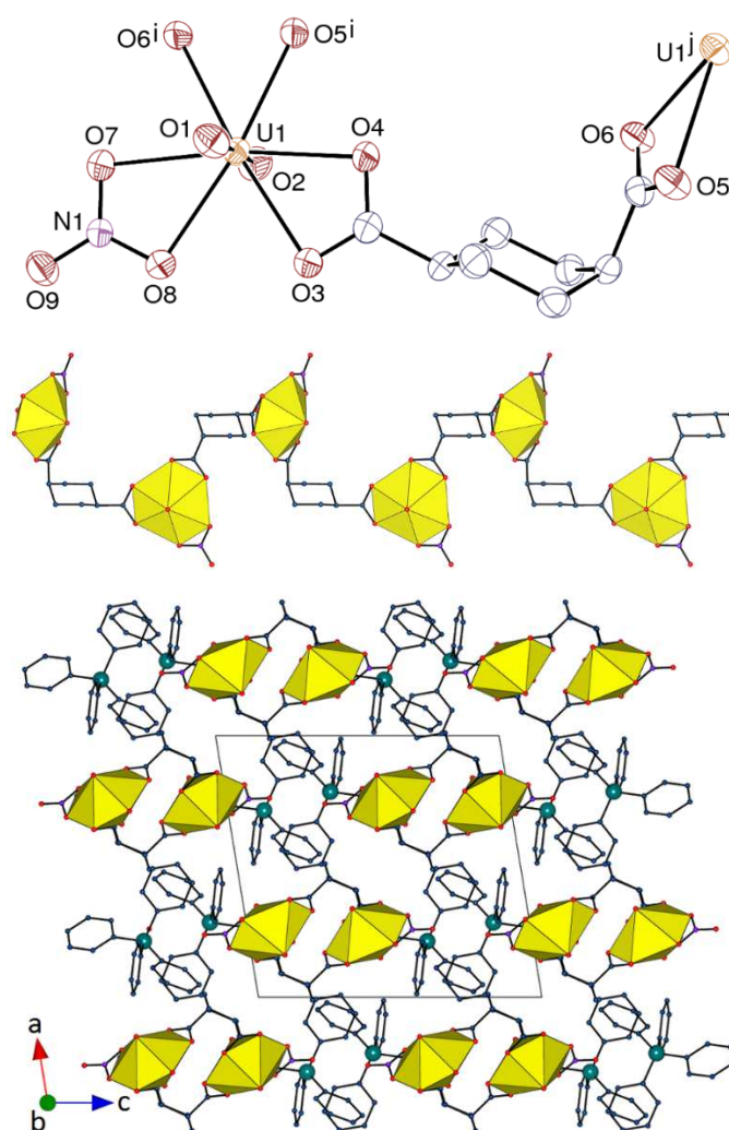
Figure 6. Top: View of compound 5 . Displacement ellipsoids are drawn at the 50% probability level. Counterions and hydrogen atoms are omitted. Symmetry codes: i = 3/2 - x, y - 1/2, 3/2 - z ; j = 3/2 - x, y + 1/2, 3/2 - z . Middle: View of the 1D helical polymer. Bottom: Packing with chains viewed end-on. Hydrogen atoms are omitted in the last two views.
