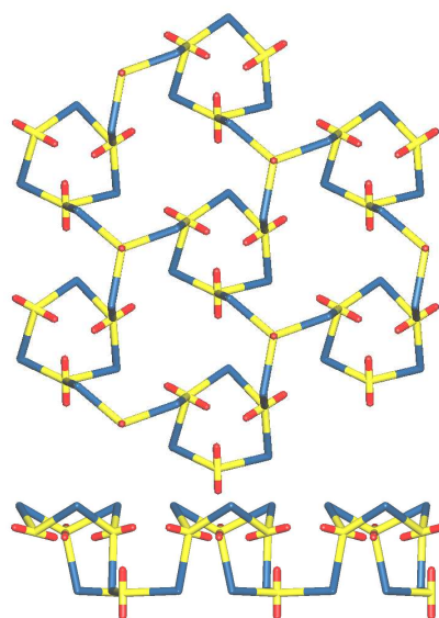
Figure 4. Simplified side-on and edge-on representations of the uranyl-based 2D network with hnb topology in compound 3 (yellow: uranium; red: oxygen; blue: centroid of the dicarboxylate ligand).
