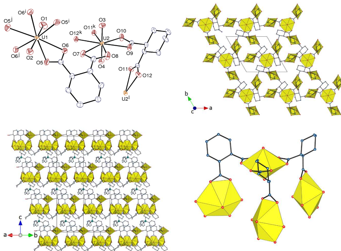
Figure 3. Top left: View of compound 3 . Displacement ellipsoids are drawn at the 30% probability level. Counterions, solvent molecules and hydrogen atoms are omitted. Symmetry codes: i = 1 - y, x - y + 1, z ; j = y - x, 1 - x, z ; k = -y, x - y, z ; l = y - x, -x, z . Top right: View of the uranyl-based 2D network. Bottom left: Packing with sheets viewed edge-on, and solvent molecules and hydrogen atoms omitted. Bottom right: Local arrangement of uranyl ions and dicarboxylate ligands around the threefold rotation axis.
