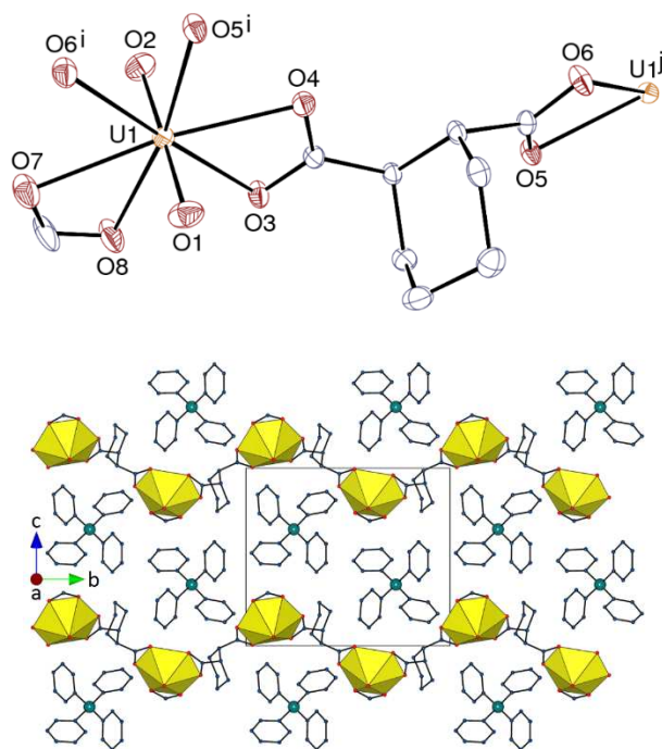
Figure 1. Top: View of compound 1 . Displacement ellipsoids are drawn at the 30% probability level. Counterions and hydrogen atoms are omitted. Symmetry codes: i = 1 - x, y - 1/2, -z ; j = 1 - x, y + 1/2, -z . Bottom: Packing with uranium coordination polyhedra colored yellow and hydrogen atoms omitted.
