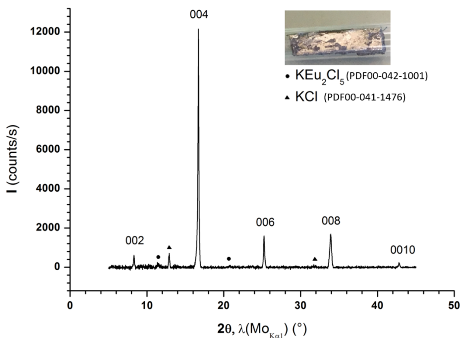
Figure 1 - 00l X-ray diffraction pattern of the first stage \text{EuC}_6\text{GIC} ( I_c = 487 pm, \lambda_{\text{MoK}\alpha 1} = 70.926 pm). A picture of the bulk sample is given in inset.
