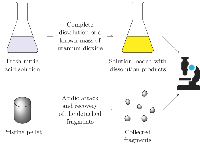
Fig. 4. Diagram of the experimental protocol for the study of the autocatalyzed reaction kinetics.
