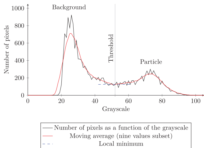
Fig. 7. Example of threshold establishing.
