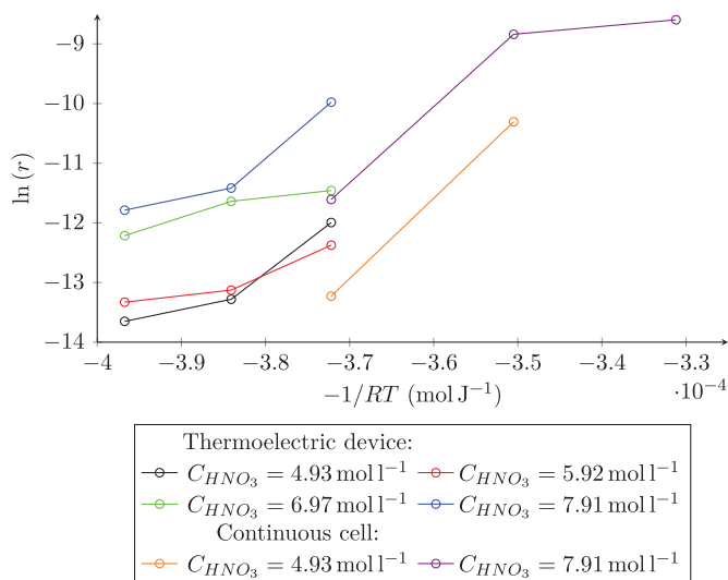
Fig. 16. Arrhenius plot of the dissolution rates.
