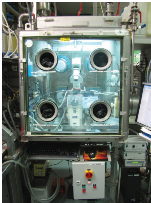
Fig. 1. Microscopy installation in the glove box.
