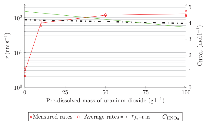
Fig. 13. Dissolution rates as a function of the pre-dissolved mass of uranium dioxide.
