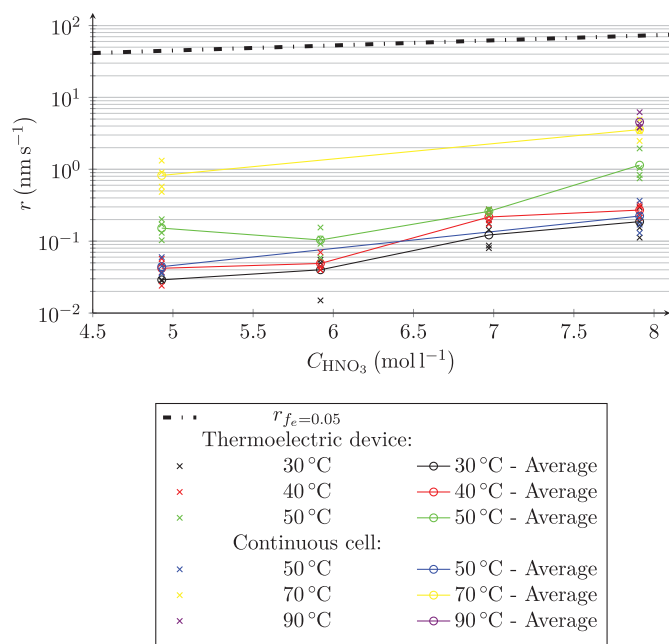
Fig. 14. Non-catalyzed dissolution rates as a function of nitric acid concentration and temperature.
