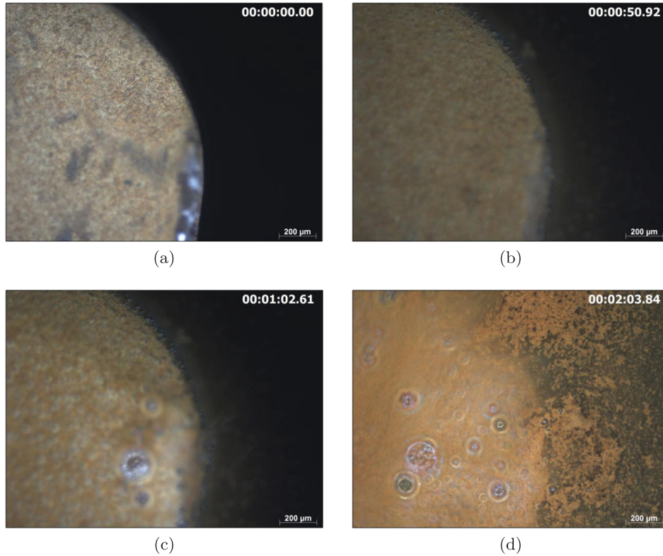
Fig. 11. Microscopic observations of the dissolution of a uranium dioxide pellet in nitric acid (corresponding times are indicated on top right of the images).
