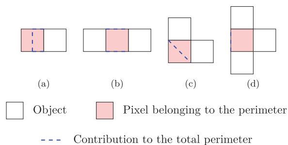
Fig. 8. Possible configurations of the neighborhood of a pixel belonging to the perimeter of the object.
