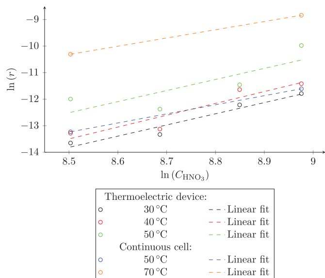
Fig. 15. Linear regression of \ln(r) as a function of \ln(C_{\text{HNO}_3}) .
