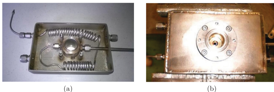
Fig. 2. Pictures of the continuous dissolution cell.
