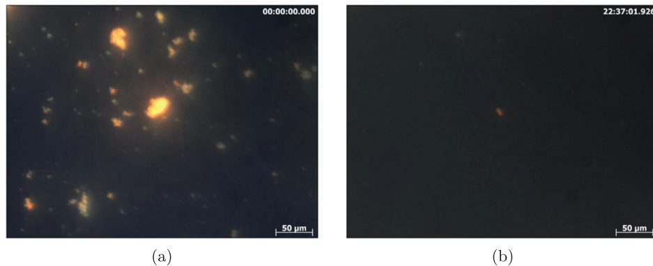
Fig. 12. Microscopic observations of the dissolution of the uranium dioxide detached fragments in nitric acid (corresponding times are indicated on top right of the images).
