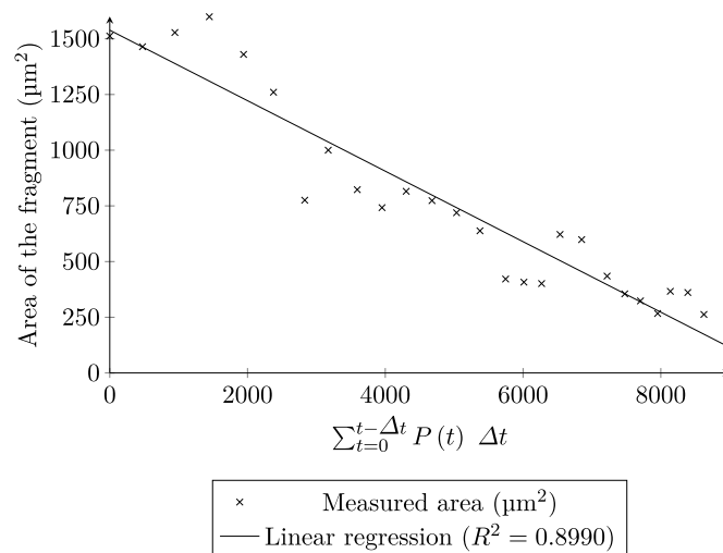
Fig. 9. Result of the processing of a set of images of a dissolving uranium dioxide fragment in 4.93 \text{ mol l}^{-1} nitric acid at \sim 343.15 \text{ K} .
