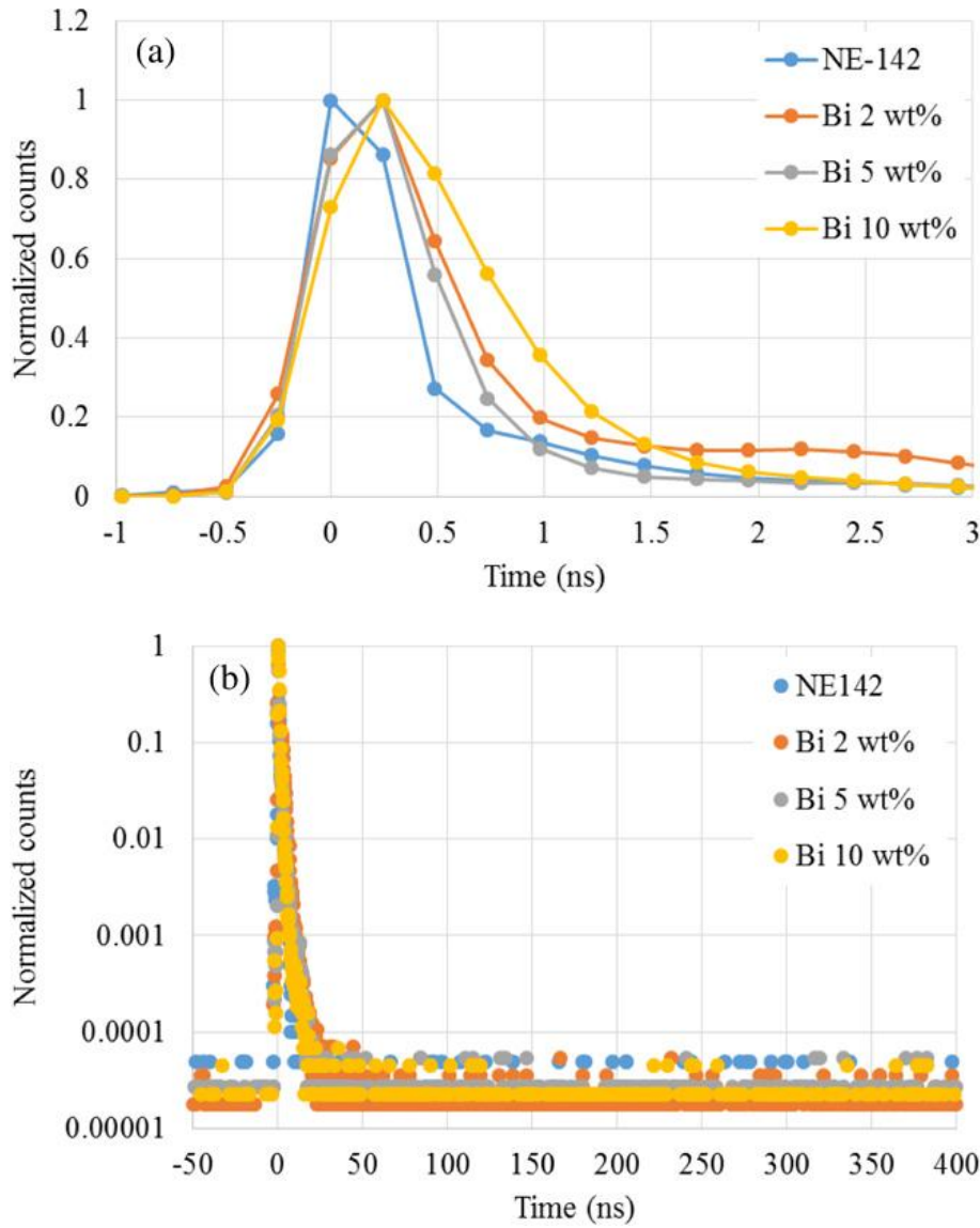
Fig. 3. Time-resolution curves of scintillation detectors equipped with sample scintillators for 67.4 keV X-ray excitation on (a) short and (b) long time scales.
