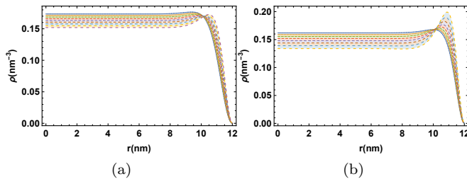
FIG. 4. Genome density profile for N = 1000 and (a) various surface charge density ( 0-0.4 e \text{ nm}^{-2} ) with salt concentration \lambda=400\text{mM} ; (b) various salt concentration ( 250-500 \text{ mM} ) with fixed surface charge \sigma = 0.4 e \text{ nm}^{-2} . Other parameters correspond to kuhn length a=1\text{nm} , excluded volume u_0=0.05\text{nm}^3 , capsid radius R=12\text{nm} .
