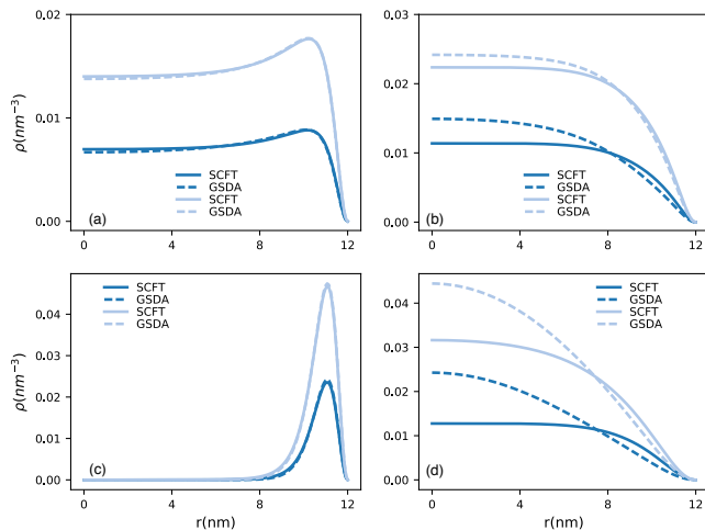
FIG. 2. Confined RNA concentration profiles with various RNA length N=50 (darker), N=100 (lighter) under SCFT calculation (solid lines) and GSDA approximation (dashed lines) with (a) linear chain charge density \tau=-1.0e , capsid surface charge density \sigma=0.8e \text{ nm}^{-2} and salt concentration \lambda=500\text{mM} ; (b) \tau=-1.0e , \sigma=0.4e \text{ nm}^{-2} , \lambda=500\text{mM} ; (c) \tau=-1.0e , \sigma=0.4e \text{ nm}^{-2} , \lambda=100\text{mM} . (d) \tau=-0.1e , \sigma=0.4e \text{ nm}^{-2} , \lambda=100\text{mM} ; Other parameters used are Kuhn length a=1\text{nm} , excluded volume u_0=0.05\text{nm}^3 , capsid radius R=12\text{nm} .
