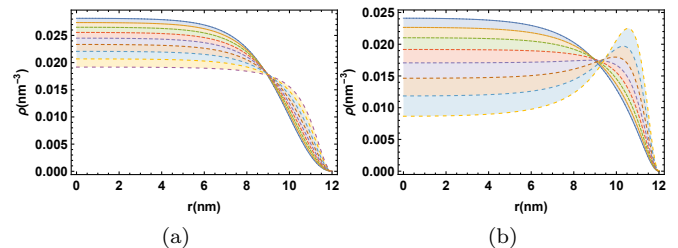
FIG. 5. Genome density profile for N = 100 and (a) various surface charge density ( 0-0.4 e \text{ nm}^{-2} ) with salt concentration \lambda=400\text{mM} ; (b) various salt concentration ( 250-500 \text{ mM} ) with fixed surface charge \sigma = 0.4 e \text{ nm}^{-2} . Other parameters correspond to a=1\text{nm} , u_0=0.05\text{nm}^3 , R=12\text{nm} .
