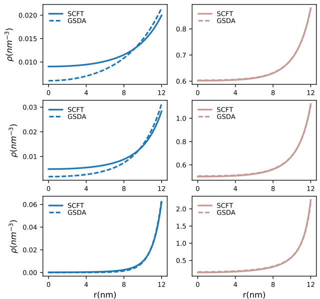
FIG. 1. Confined RNA density profile vs r the distance from the capsid center for various extrapolation lengths, \kappa^{-1}=10.0, 5.0, 2.0 nm for top to the bottom of the figure. The total monomer number is N=100 (left), N=5000 (right).
