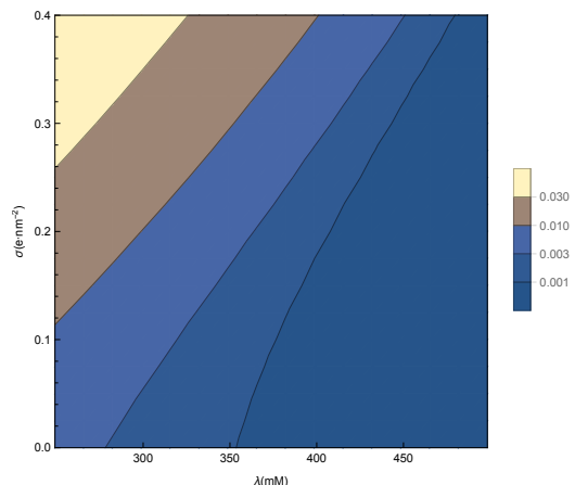
FIG. 3. Genome excess phase diagram with respect to salt concentration and capsid surface charge density. The white shade corresponds to the region with the maximum genome density and black to the depletion regime next to the wall. Other parameters used are N = 500 , a=1\text{nm} , u_0=0.05\text{nm}^3 , R=12\text{nm} .
