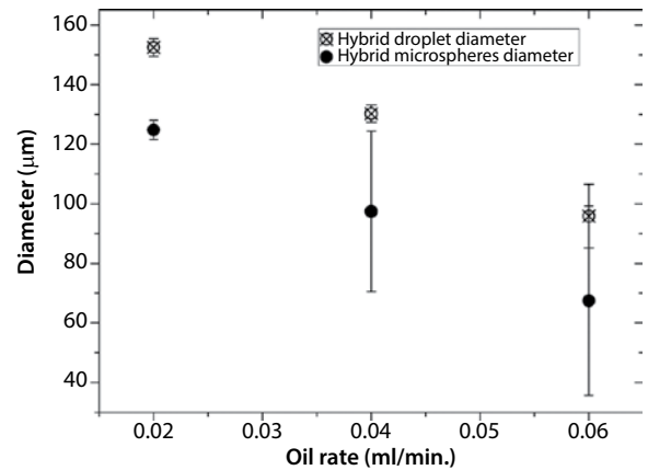
Figure 4 Size of hybrid chitosan-collagen emulsion droplets (crossed open circle) and microspheres after ammonia vapors (solid circles) as a function of oil flow rate at constant chitosan solution flow rate ( 0.002 \text{ ml}\cdot\text{min}^{-1} ). Chip 100 \times 100 \mu\text{m}^2 cross design.
