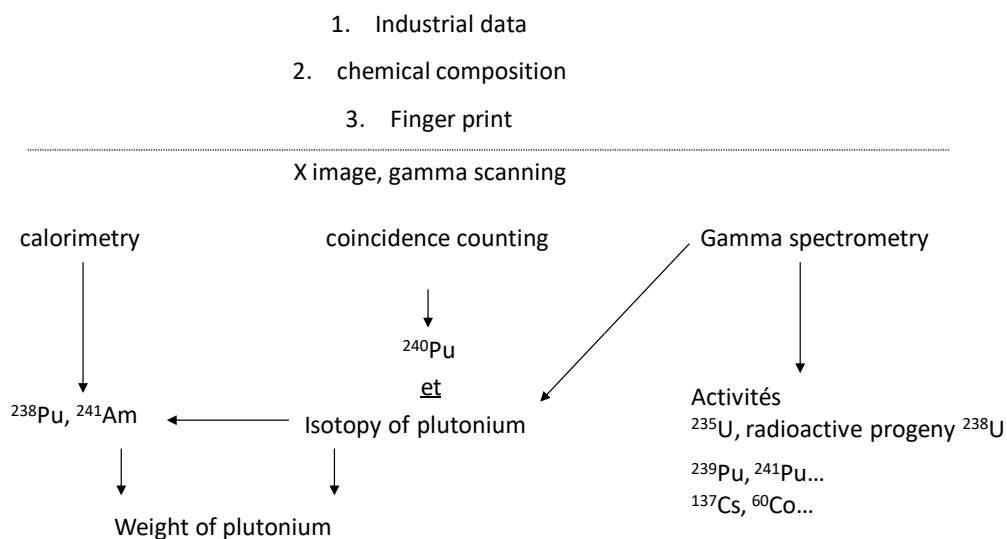
Figure 10: Flow sheet of non destructive analysis method combinations (process control: package)
