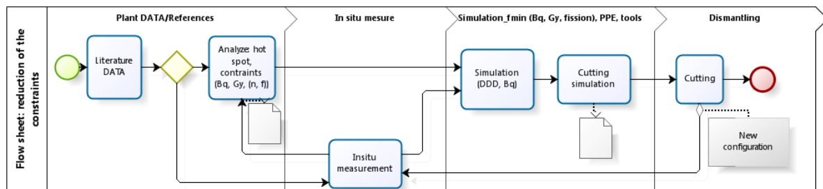
Figure 2: Simplified flow sheet for the minimization of constraint parameters, or operational functional architecture of the reduction function
