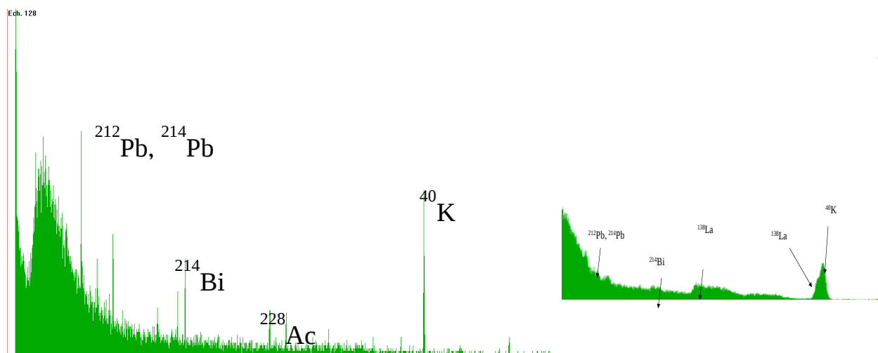
Figure 13: (left) gamma spectrum of a concrete surface - GeHp detector, 40% relative yield; (right) gamma spectrum of a concrete surface with a LaBr3 3x3 inch detector.
