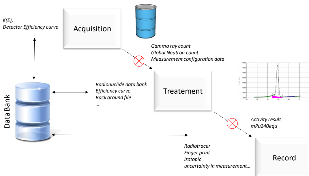
Figure 11: Functional flow sheet of an Information System (IS) for nuclear waste package management in the CEA
