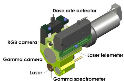
Figure 5: Example of a module grouping instruments for the location and radiological characterization of hot spots (DUCROS, HAUSER, Majhoubi, & GIRONES, 2016)
