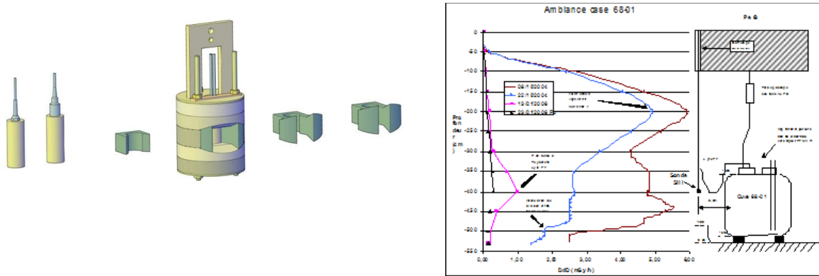
Figure 7: Example of a modular collimation used to monitor component cleanup within multi-source scenes (GIRONES P. , 2009)
