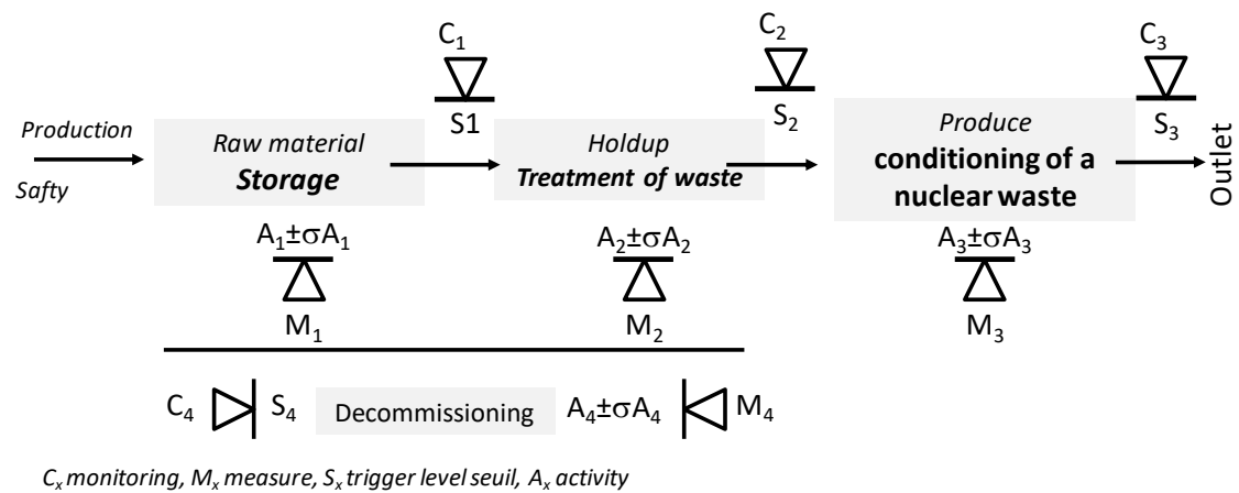
Figure 3: Functional block flow chart for waste treatment in three phases - A_x : activity in Bq, M_x : measurement point, C_1 : check/control point, S_x : threshold in Bq)
