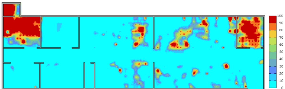
Figure 14: Risk of exceeding (in %) a threshold of 150 cps, for the signal \square\square\square , uranium contamination (DESNOYER, 2010)
