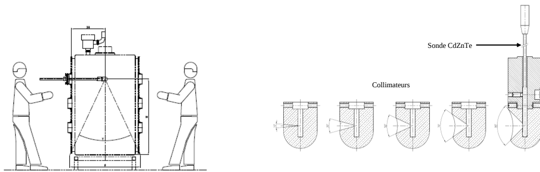
Figure 8: Positioning system for the detector in a glove box - Collimators with solid angles from 10° to 90° (BRENNEIS & GIRONES, 2011)
