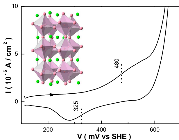
Fig. 9. Cyclic voltammograms for a 64 nm-thick \text{SrIrO}_3 thin film ( S = 5.2 \text{ mm}^2 ), in 1 M KOH ( 2.3 \times 10^{-3} \text{ V/s} ). The structure is from Ref. [34].
